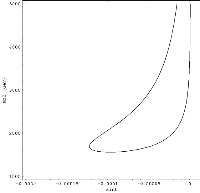
FIG. 2. Contour plot displaying the allowed region for \sin \theta vs M_{Z_2} at 95% C.L.
