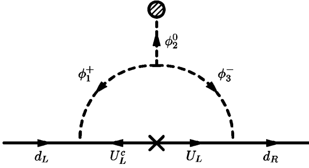
FIG. 1. A One-loop diagram contributing to the radiative generation of the down quark mass.
