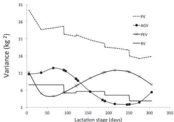
Figure 1. Additive genetic (AGV), phenotypic (PV), permanent environmental (PEV), and residual variances (RV) obtained throughout lactation of Holstein cows in Antioquia.
