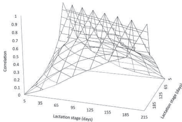
Figure 4. Phenotypic correlations between the different days of lactation for milk production of Holstein cattle in Antioquia, obtained with a random regression model.
