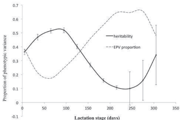
Figure 2. Heritabilities (with standard errors) and permanent environment variance (PEV) ratio throughout lactation of Holstein cattle in Antioquia.
