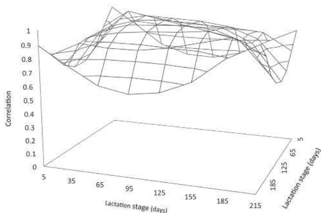
Figure 3. Genetic correlations for days in milk obtained with a random regression model for milk yield of Holstein cattle in Antioquia.
