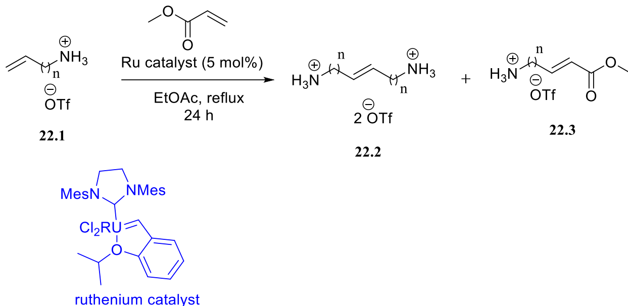
Scheme 28: Cross metathesis of alkenyl amine with acrylate
