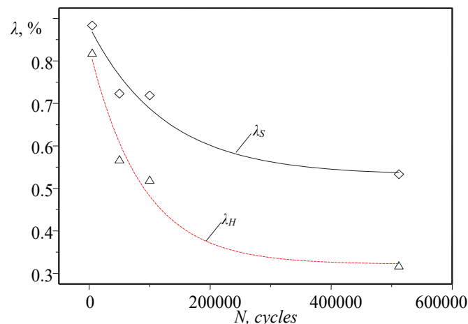
Figure 4: Dependence of the relative damage indicators \lambda_S and \lambda_{HI} versus the number loading cycles of the sensor.
