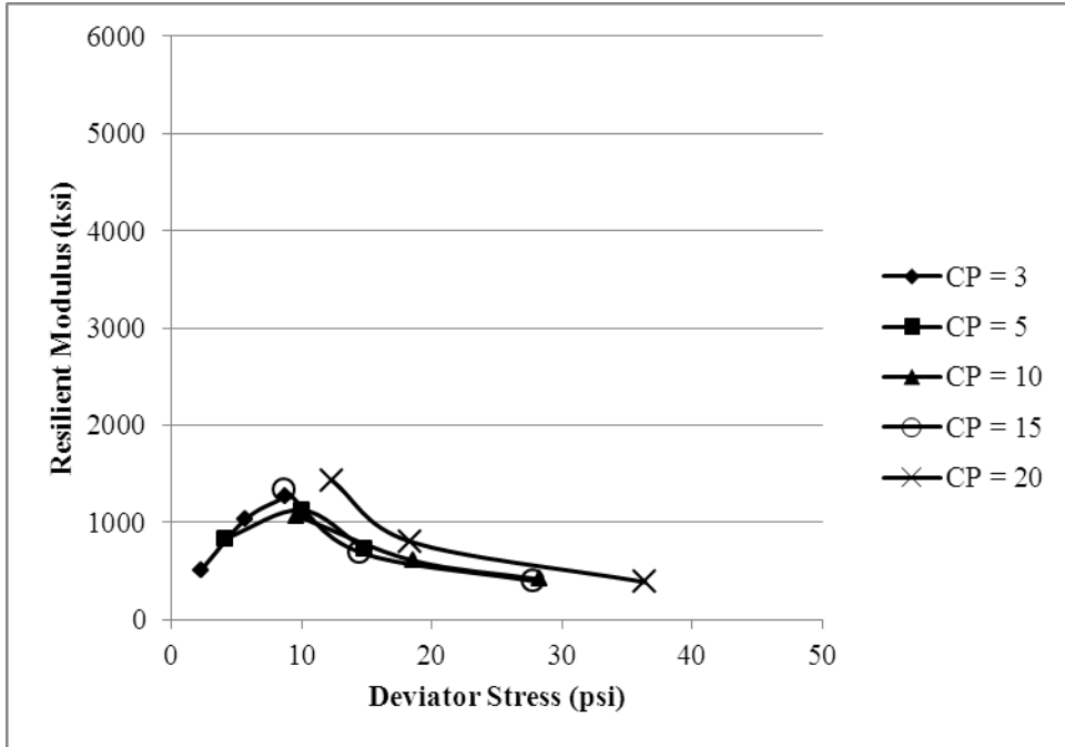
Figure 4.20 M_R for FC = 6%, MC = 3.3%, medium gradient, -1^\circ\text{C}
