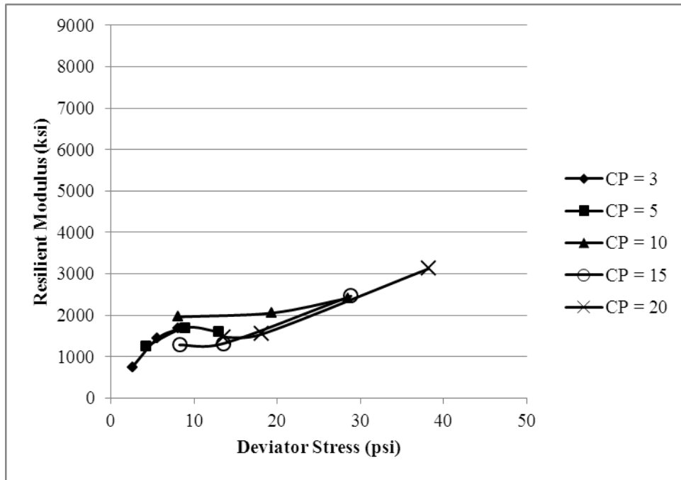
Figure I.1. M_R for FC = 6%, MC = 3.3%, Low Gradient, -1\text{ }^\circ\text{C}
