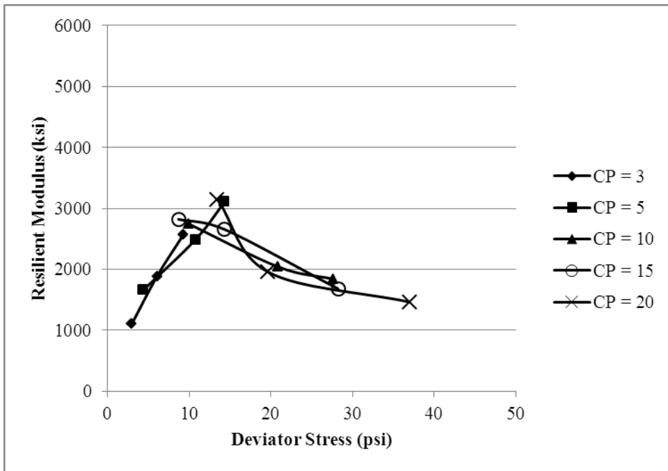
Figure 4.21 M_R for FC = 6%, MC = 5.3%, medium gradient, -1^\circ\text{C}
