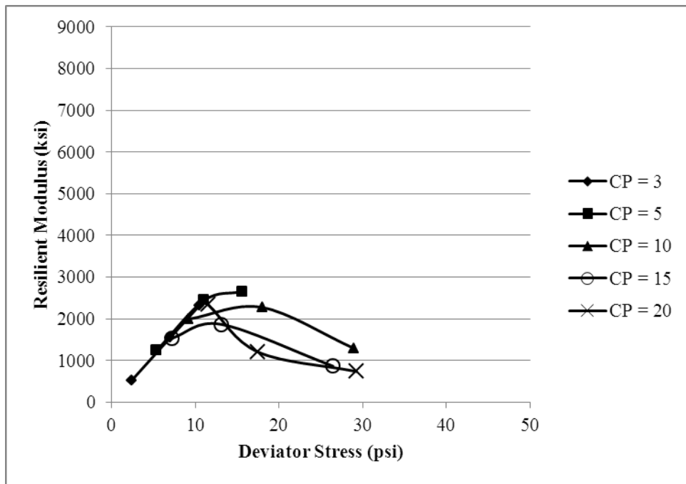
Figure I.8. M_R for FC = 12%, MC = 3.3%, Medium Gradient, -1\text{ }^\circ\text{C}
