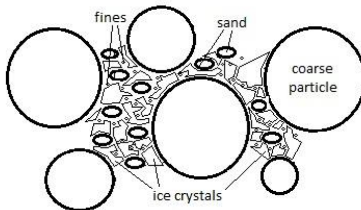
Figure 4.26 Soil particles at -1^{\circ}\text{C}
