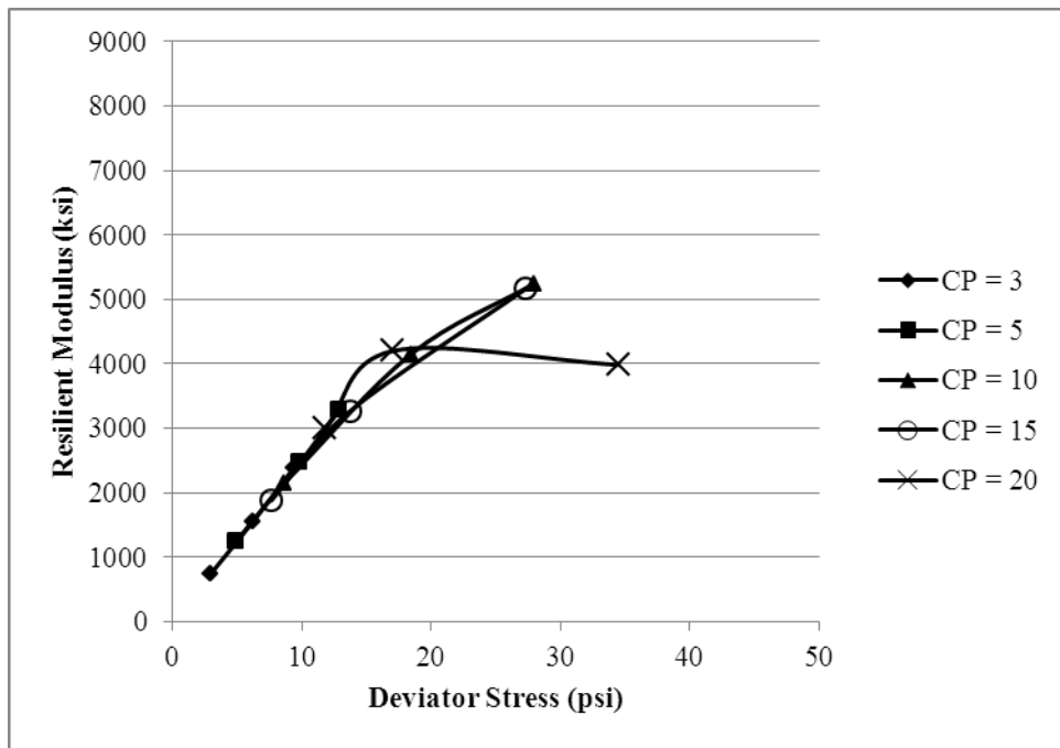
Figure I.16. M_R for FC = 12%, MC = 5.3%, High Gradient, -1\text{ }^\circ\text{C}
