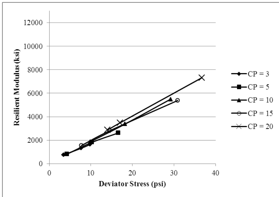
Figure H.6. M_R for FC = 12%, MC = 6%, Low Gradient, -5\text{ }^\circ\text{C}
