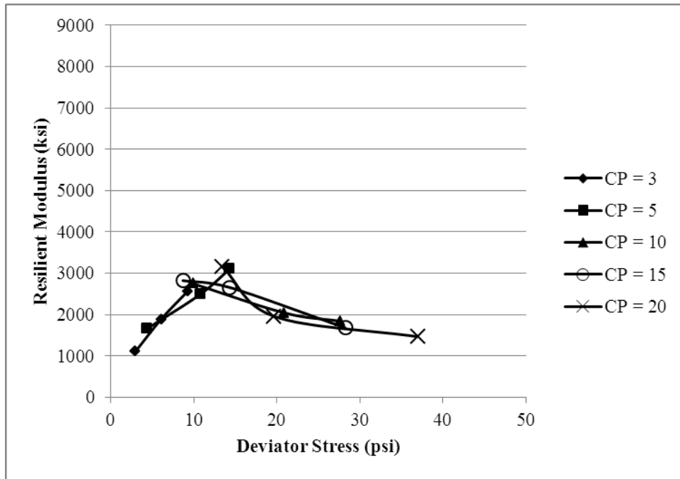
Figure I.9. M_R for FC = 6%, MC = 5.3%, Medium Gradient, -1\text{ }^\circ\text{C}
