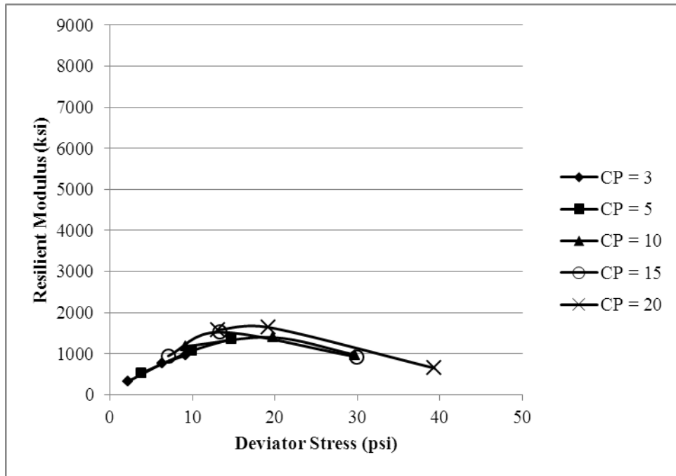
Figure I.5. M_R for FC = 6%, MC = 6%, Low Gradient, -1\text{ }^\circ\text{C}
