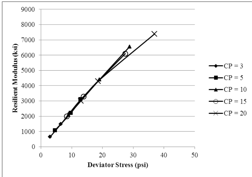
Figure I.15. M_R for FC = 6%, MC = 5.3%, High Gradient, -1\text{ }^\circ\text{C}
