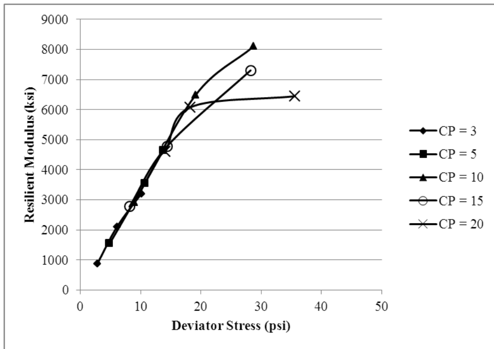
Figure I.18. M_R for FC = 12%, MC = 6%, High Gradient, -1\text{ }^\circ\text{C}
