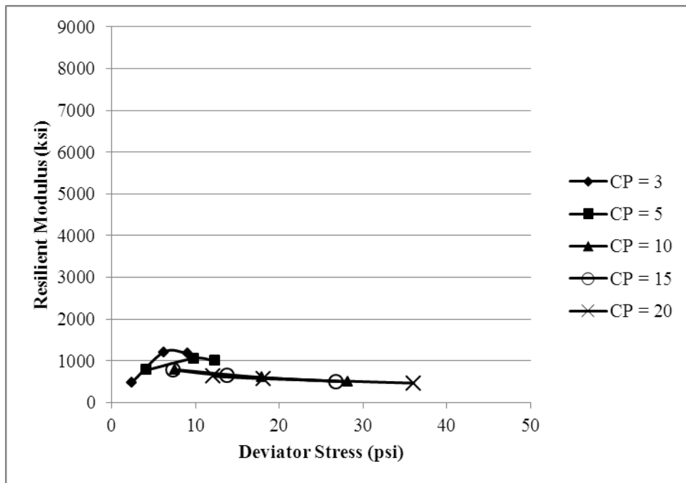
Figure I.2. M_R for FC = 12%, MC = 3.3%, Low Gradient, -1\text{ }^\circ\text{C}
