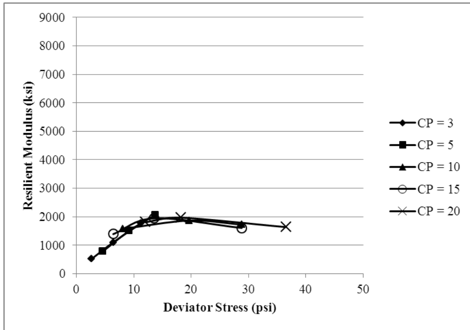
Figure I.3. M_R for FC = 6%, MC = 5.3%, Low Gradient, -1\text{ }^\circ\text{C}
