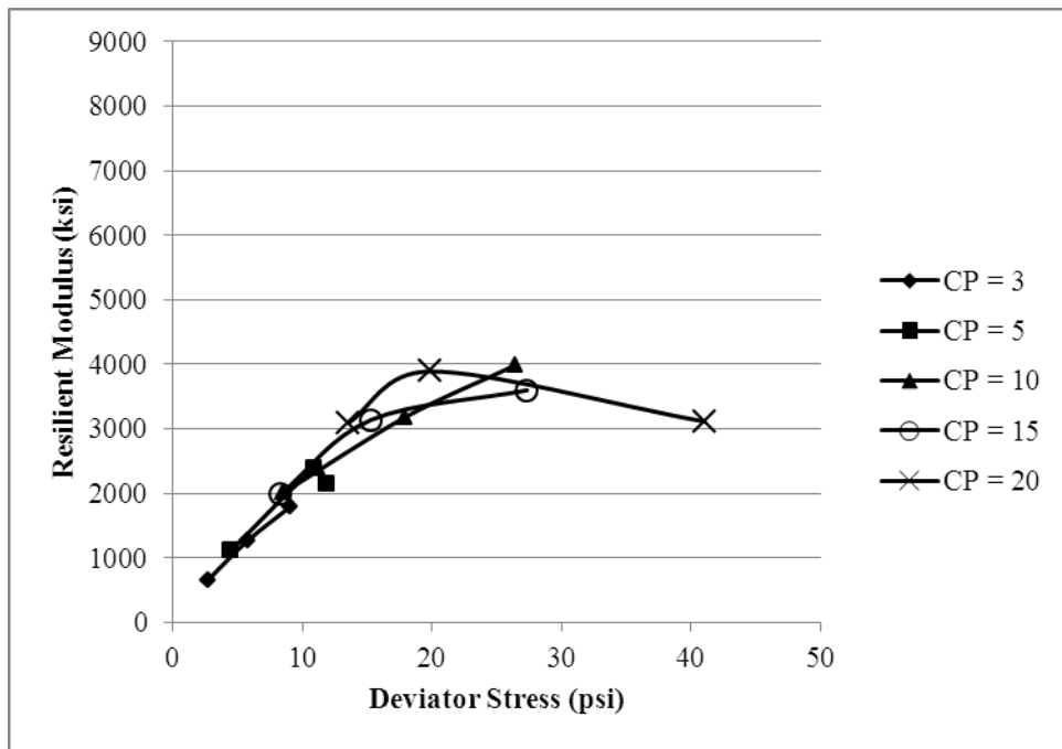
Figure I.6. M_R for FC = 12%, MC = 6%, Low Gradient, -1\text{ }^\circ\text{C}
