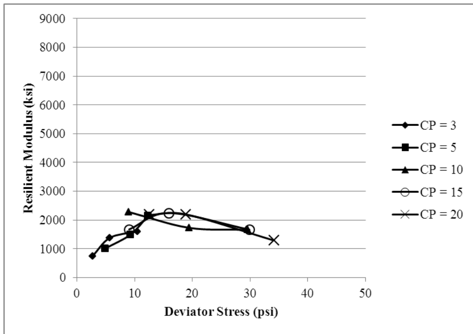
Figure I.4. M_R for FC = 12%, MC = 5.3%, Low Gradient, -1\text{ }^\circ\text{C}
