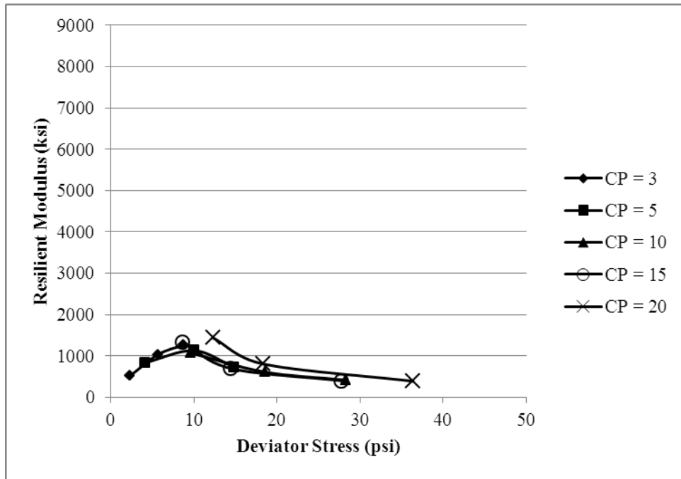
Figure I.7. M_R for FC = 6%, MC = 3.3%, Medium Gradient, -1\text{ }^\circ\text{C}
