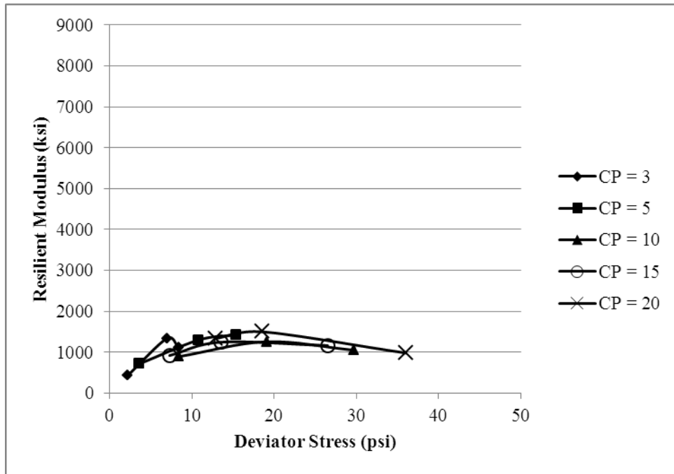
Figure I.17. M_R for FC = 6%, MC = 6%, High Gradient, -1\text{ }^\circ\text{C}
