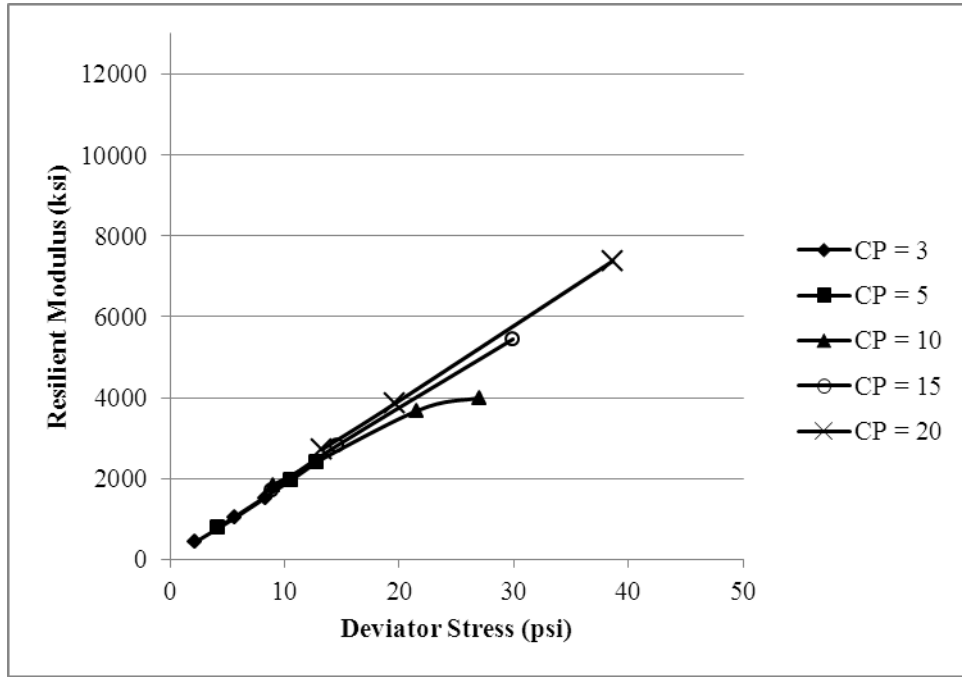
Figure H.5. M_R for FC = 6%, MC = 6%, Low Gradient, -5\text{ }^\circ\text{C}
