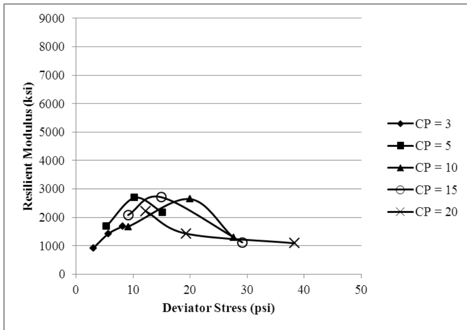
Figure I.10. M_R for FC = 12%, MC = 5.3%, Medium Gradient, -1\text{ }^\circ\text{C}
