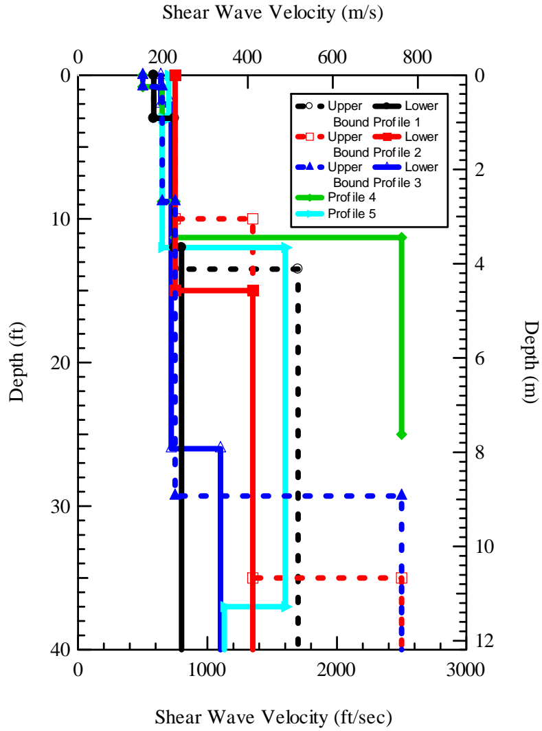
Figure 123 Shear wave velocity profile comparison for Site 29, 0-40ft (WRRC).
