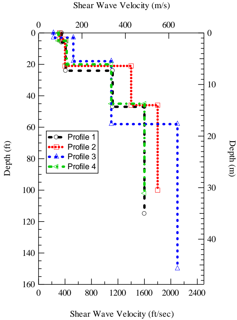
Figure 13 Shear wave velocity profile comparison for Site 8 (CRREL).
