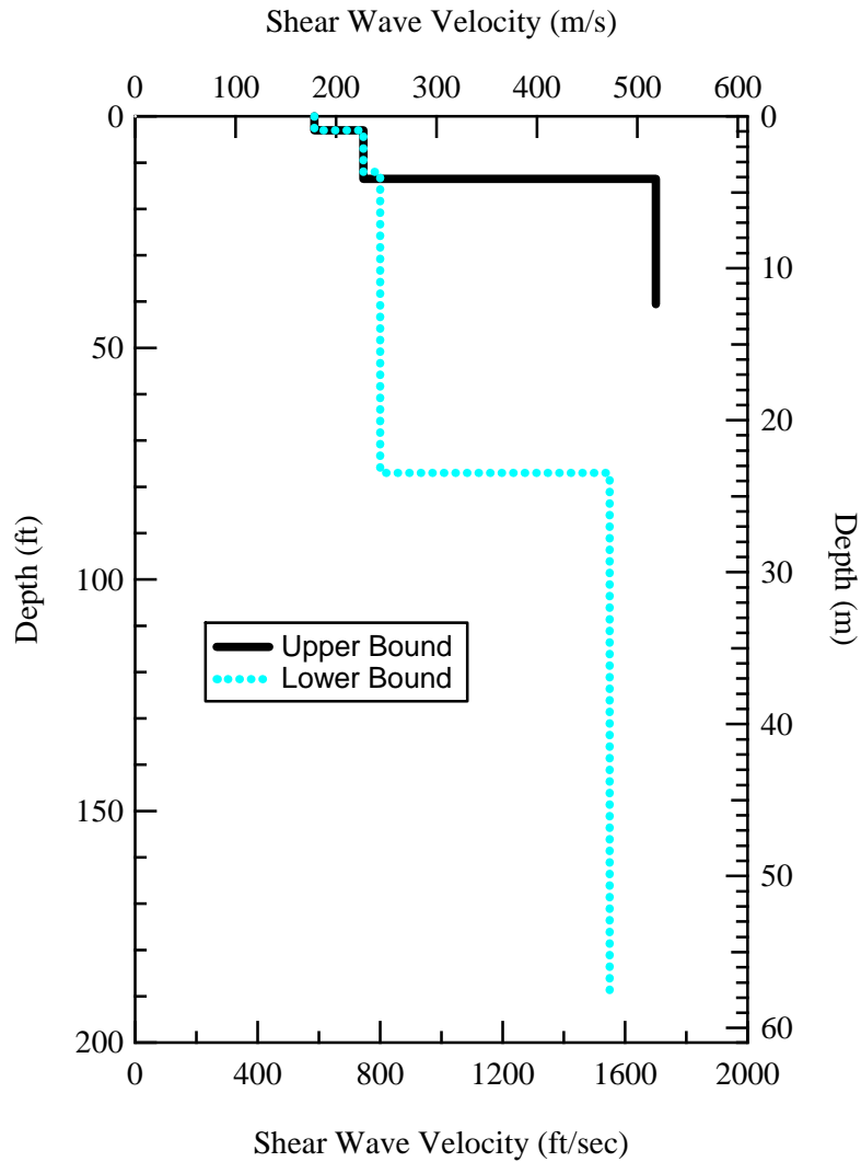
Figure 114 Shear wave velocity profile for Array #1 at Site 29 (WRRC).
