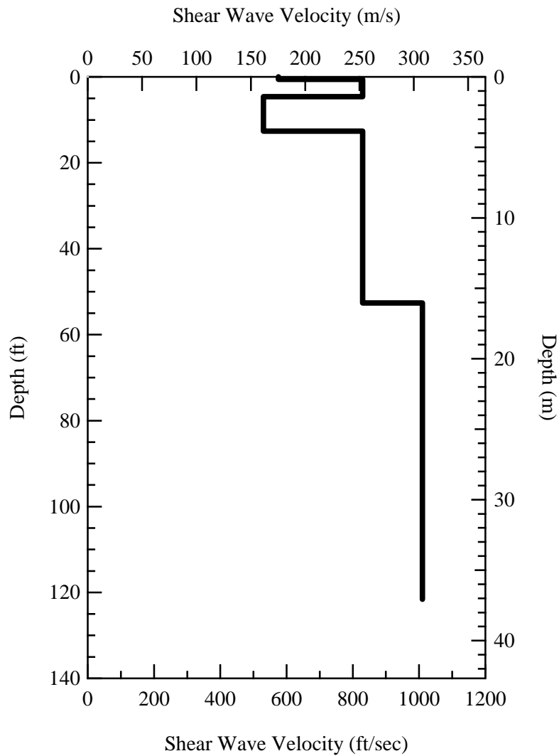
Figure 90 Shear wave velocity profile for Site 22 (Sadlers).
