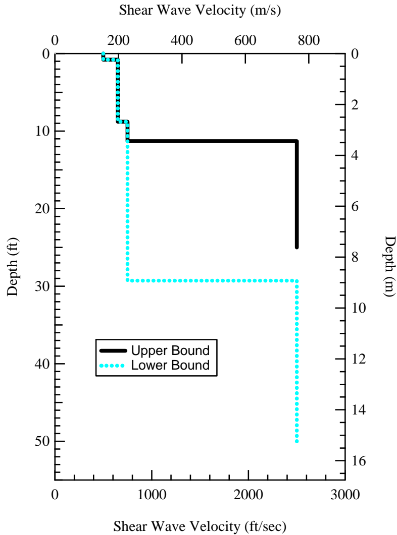
Figure 118 Shear wave velocity profile for Array #3 at Site 29 (WRRC).
