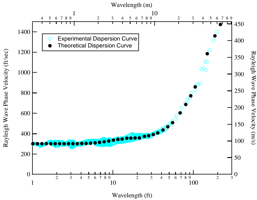
Figure 5 Experimental and theoretical dispersion curve for Array #2 at Site 8 (CRREL)..
