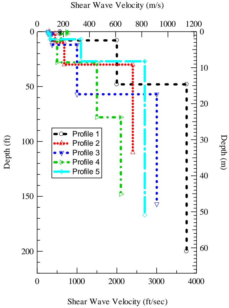
Figure 11 Shear wave velocity profile comparison for Site 6 (CCHRC).
