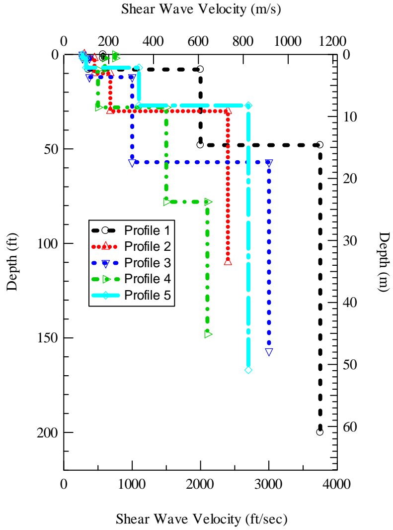
Figure 34 Shear wave velocity profile comparison for Site 6 (CCHRC).
