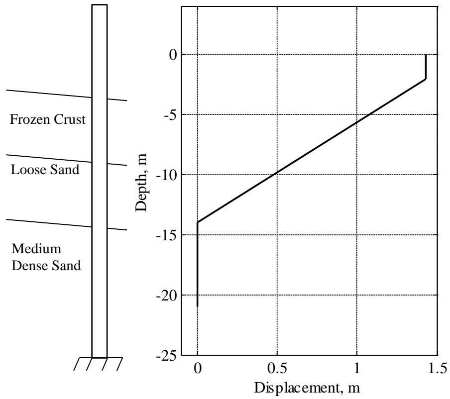
Figure 3.13. Lateral spreading load of the p - y approach for the shake table experiment modeling
