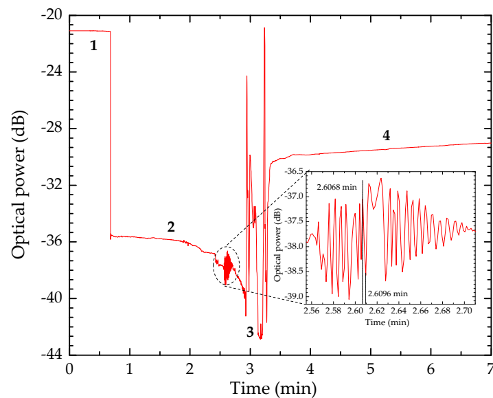
Figure 7. Monitoring of the crystallization process. (1) Addition of the paracetamol sample; (2) air exposure; (3) initiation of crystallization process; (4) stabilization, (zoom in between the steps (2) and (3)).
