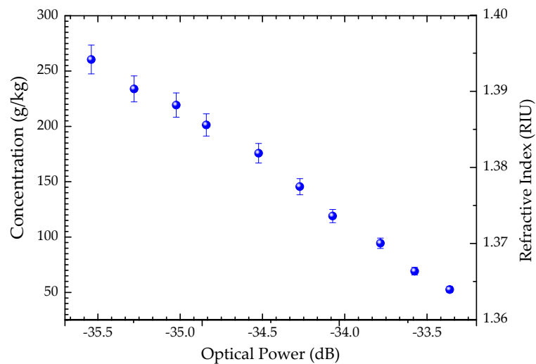
Figure 3. Optical power dependence on paracetamol concentration and respective refractive index.
