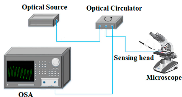
Figure 5. Experimental setup for paracetamol crystallization process monitoring.
