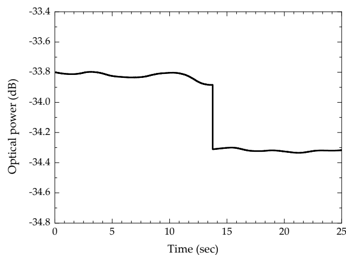
Figure 4. Step technique to estimate the resolution of the sensor.
