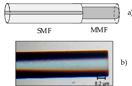
Figure 1. Schematic diagram of the sensor structure (a) and a microscope image (b).
