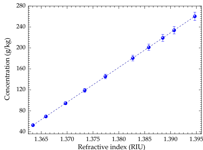
Figure 2. Paracetamol concentration dependence on the refractive index.
