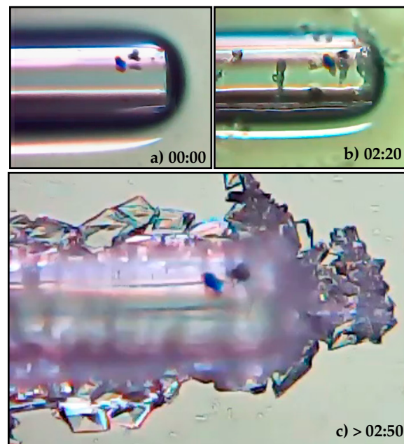
Figure 6. Crystallization process of paracetamol (video online) (a) Liquid paracetamol solution in contact with the MMF-tip sensor, (b) beginning of the paracetamol crystallization with continuous exposure to air and (c) full evaporation of the liquid solution and formation of crystalline structures of paracetamol.
