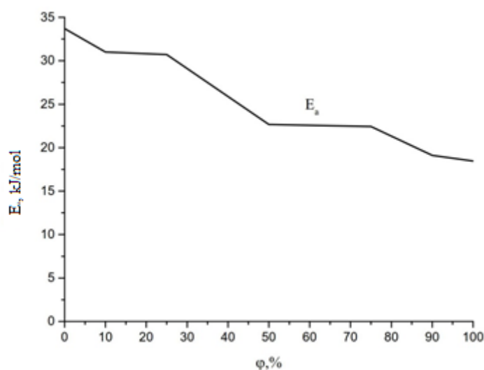
Figure 1. Activation energy during thermal decomposition of composite fuels compared to the initial coal ( \phi – wood concentration)
