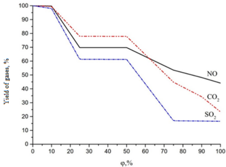
Figure 2. Concentration of released gases during thermal decomposition of composite fuels vs. pure coal ( \varphi – wood concentration)
