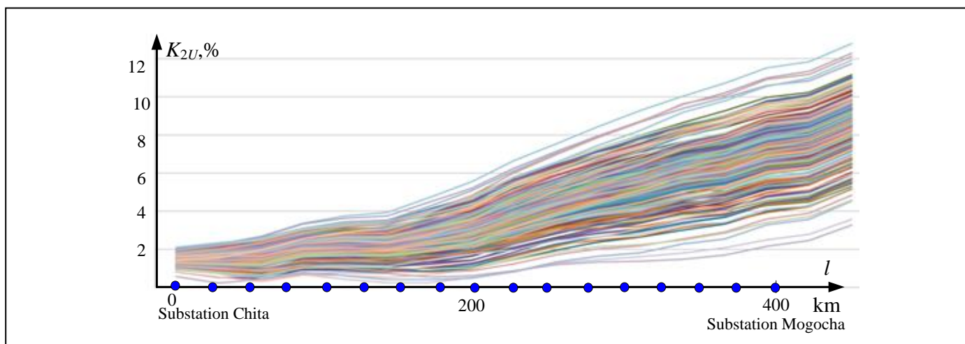
Fig. 3. Change of negative voltage unbalance ratio (600 experiments)
