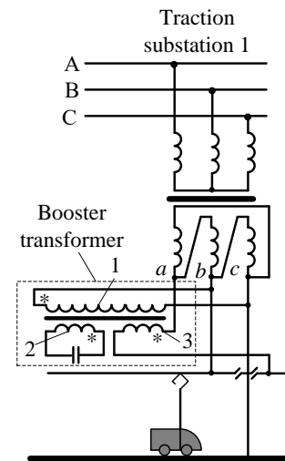
Fig.4. Connection scheme of the booster transformer
