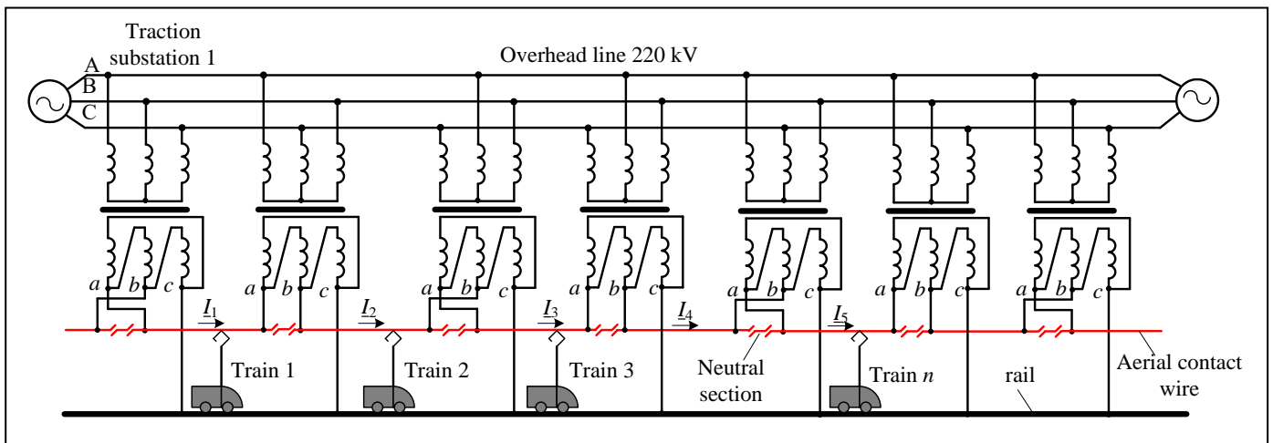
Fig. 1. Connection scheme of traction substations to the longitudinal power supply line
