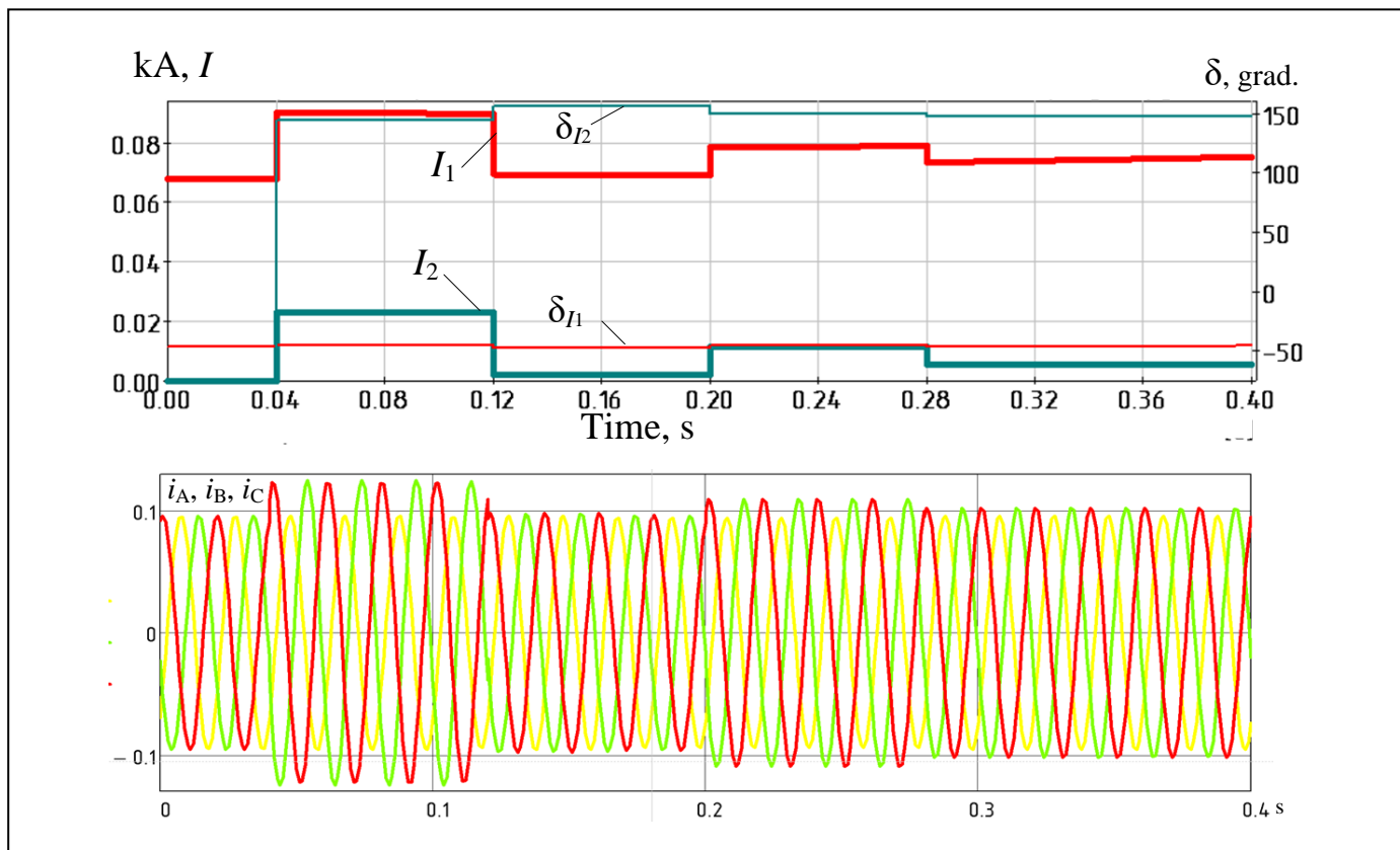
Fig. 2. Change of PS and NS currents when connecting a train on a given segment of the railway
