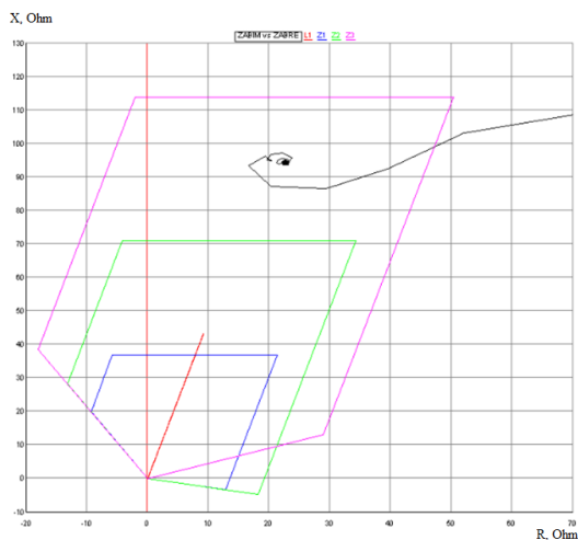
Fig. 5 Phase-to-phase fault, node 3
