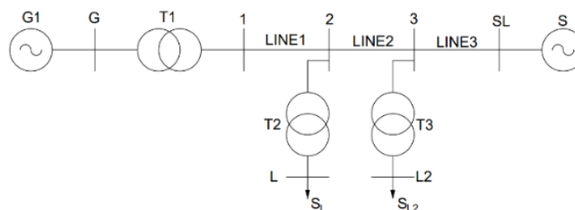
Fig. 1 Experimental power grid scheme
