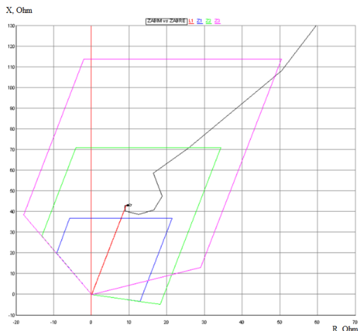
Fig. 4 Phase-to-phase fault, node 2
