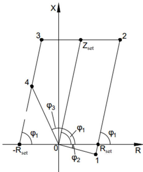
Fig. 2 Quad characteristic general form
