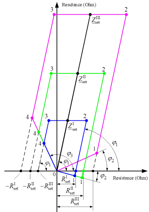
Fig. 2. Distance protection polygonal characteristics
