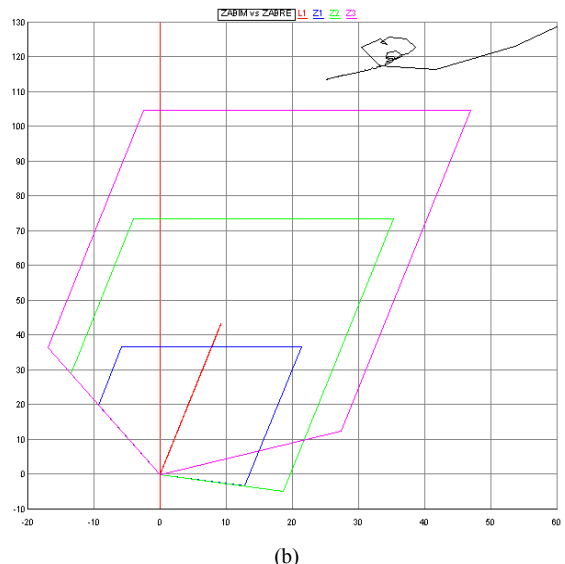
Fig. 7. Hodograph of the phase A impedance with a 3LG fault (a) and impedance between phases A and B with a LL fault (b) at the end of the adjacent line L2 at wind speed 50 km/h \approx 14 m/s
