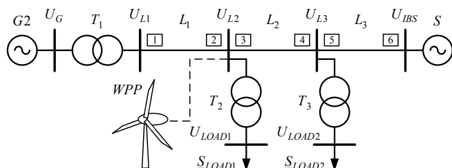
Fig. 4. Experimental scheme with the installation of wind turbines at the end of the protected power line L1
