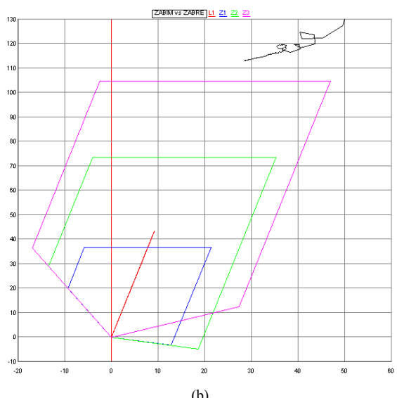
Fig. 6. Hodograph of the phase A impedance with a 3LG fault (a) and impedance between phases A and B with a LL fault (b) at the end of the adjacent line L2 at wind speed 36 km/h = 10 m/s
