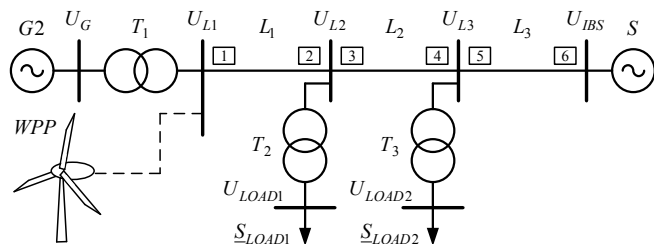
Fig. 3. Experimental scheme with the installation of wind turbines at the beginning of the protected power line L1
