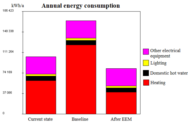
Fig. 8. Outputs from the energy modeling of building 2
