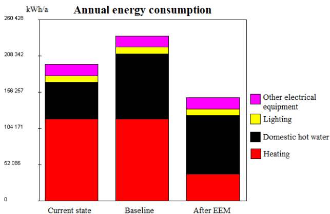
Fig. 9. Outputs from the energy modeling of building 3
