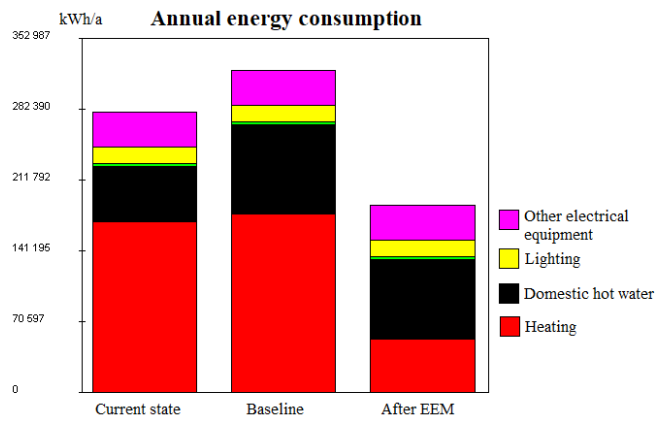
Fig. 10. Outputs from the energy modeling of building 4
