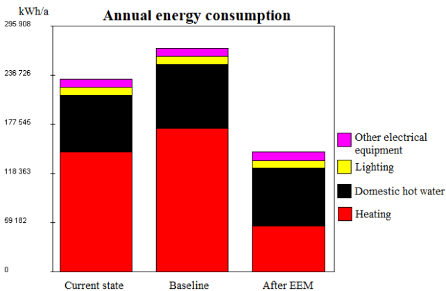
Fig. 7. Outputs from the energy modeling of building 1
