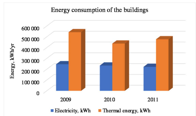
Fig. 5. Yearly annual energy consumption of the buildings
