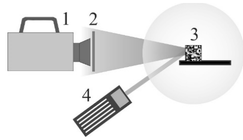
Fig. 1. Experimental scheme. 1 - high-speed monochrome camera with objective, 2 - 532 nm narrow-band filter, 3 - cuboid nanopowder, 4 - Nd:YAG laser.
