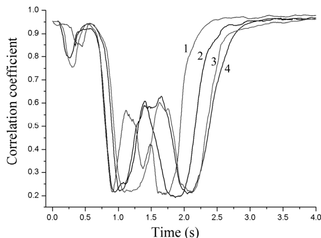
Fig. 6. Time dependences of the correlation coefficient during the combustion of the mixture of aluminium and iron nanopowders.
