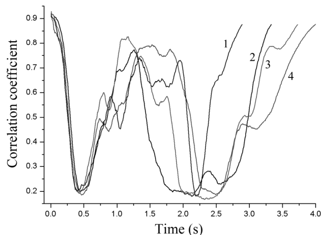
Fig. 5. Time dependences of the correlation coefficient during the combustion of four aluminium nanopowder samples.
