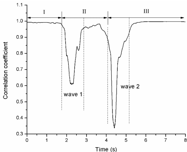
Fig. 4. The schematic time dependence of the correlation coefficient during the aluminium nanopowder combustion.
