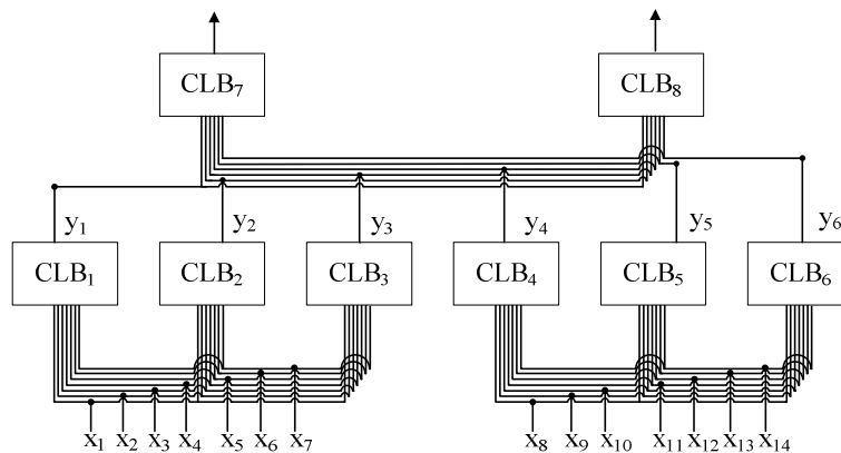
Fig. 3. The new checker of the (7, 14)-code.
