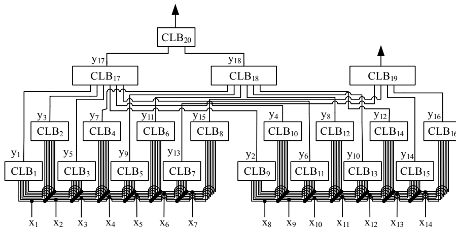
Fig. 2. The checker of the (7, 14)-code.
