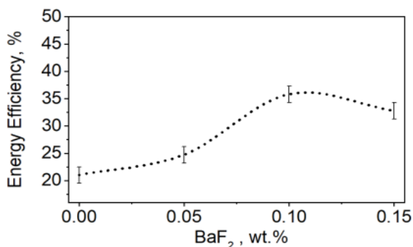
Fig. 8. Dependence of energy efficiency from barium fluoride flux
