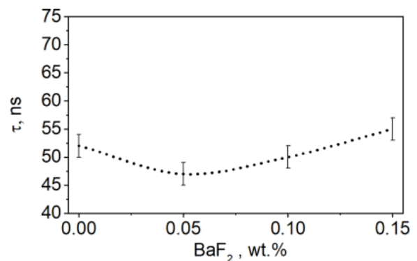
Fig. 6. Dependence of decay times from barium fluoride flux
