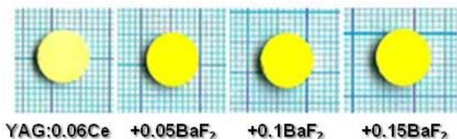
Fig. 1. Sintered ceramic samples.
