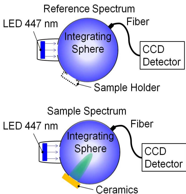
Fig. 2. Method of measuring the energy efficiency.
