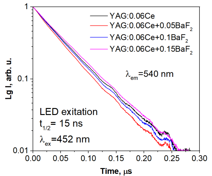
Fig. 5. Luminescence decay curves.
