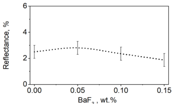
Fig. 7. Dependence of reflectance values from barium fluoride flux
