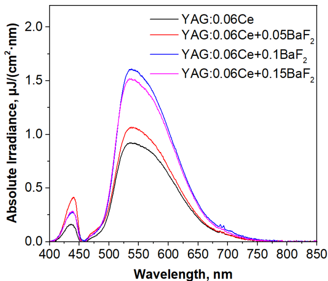
Fig. 4. Photoluminescence spectra ( \lambda_{ex} = 447 nm)
