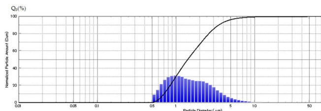
Fig. 2. Grain-size waste distribution
