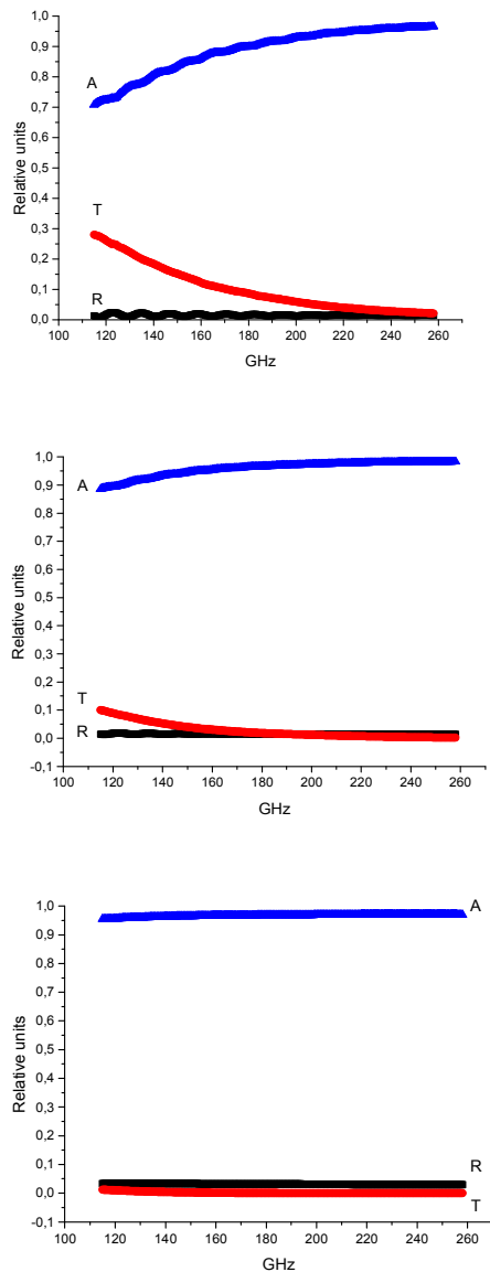
Fig.5. The dependence of the absorption (A), reflection (R) and transmission (T) coefficients of the frequency 120 - 260 GHz for the sample without waste (top) and with a waste of 30% (bottom)
