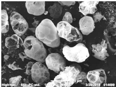
Fig. 1. Electronic micrograph of perlite microspheres
