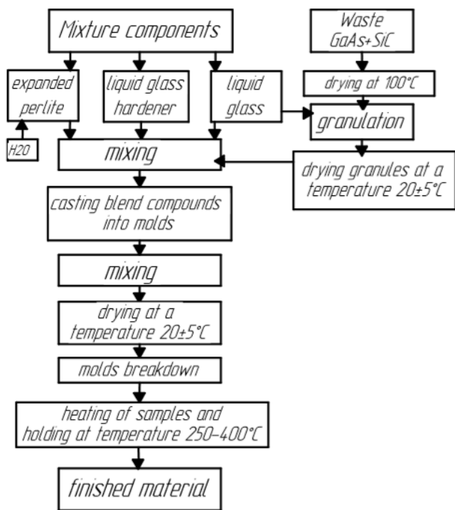
Fig.3. Technological scheme for obtaining electromagnetic radiation absorber with waste of semiconductor manufacturing
