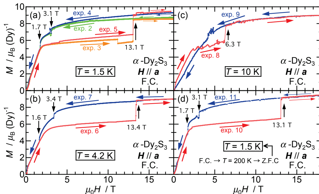
Figure 3. Magnetization curves along the a -axis of \alpha - \text{Dy}_2\text{S}_3 single crystal at some temperatures. The curves in the figures of (a)-(c) are obtained after field cooling shown in Fig. 2. Before the exp. 10 shown in the figure (d) was performed, the sample had been warmed up to 200 K and then cooled down to 1.5 K in no magnetic field.
