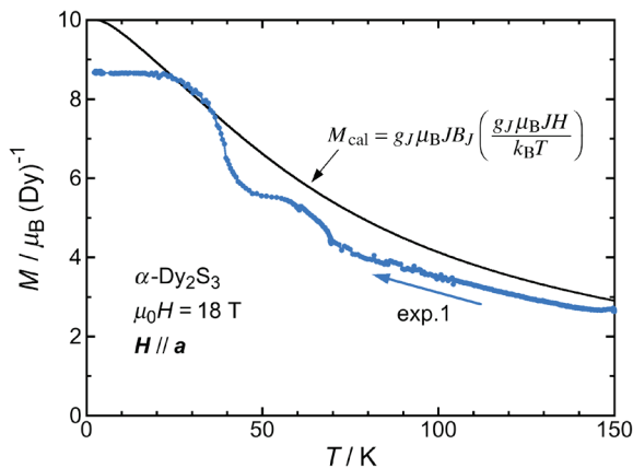
Figure 2. Temperature dependence of the magnetization per one Dy atom on the cooling process in the field of 18 T along the a -axis of \alpha -Dy 2 S 3 single crystal. The calculated M(T) curve for free Dy 3+ ion is also shown.
