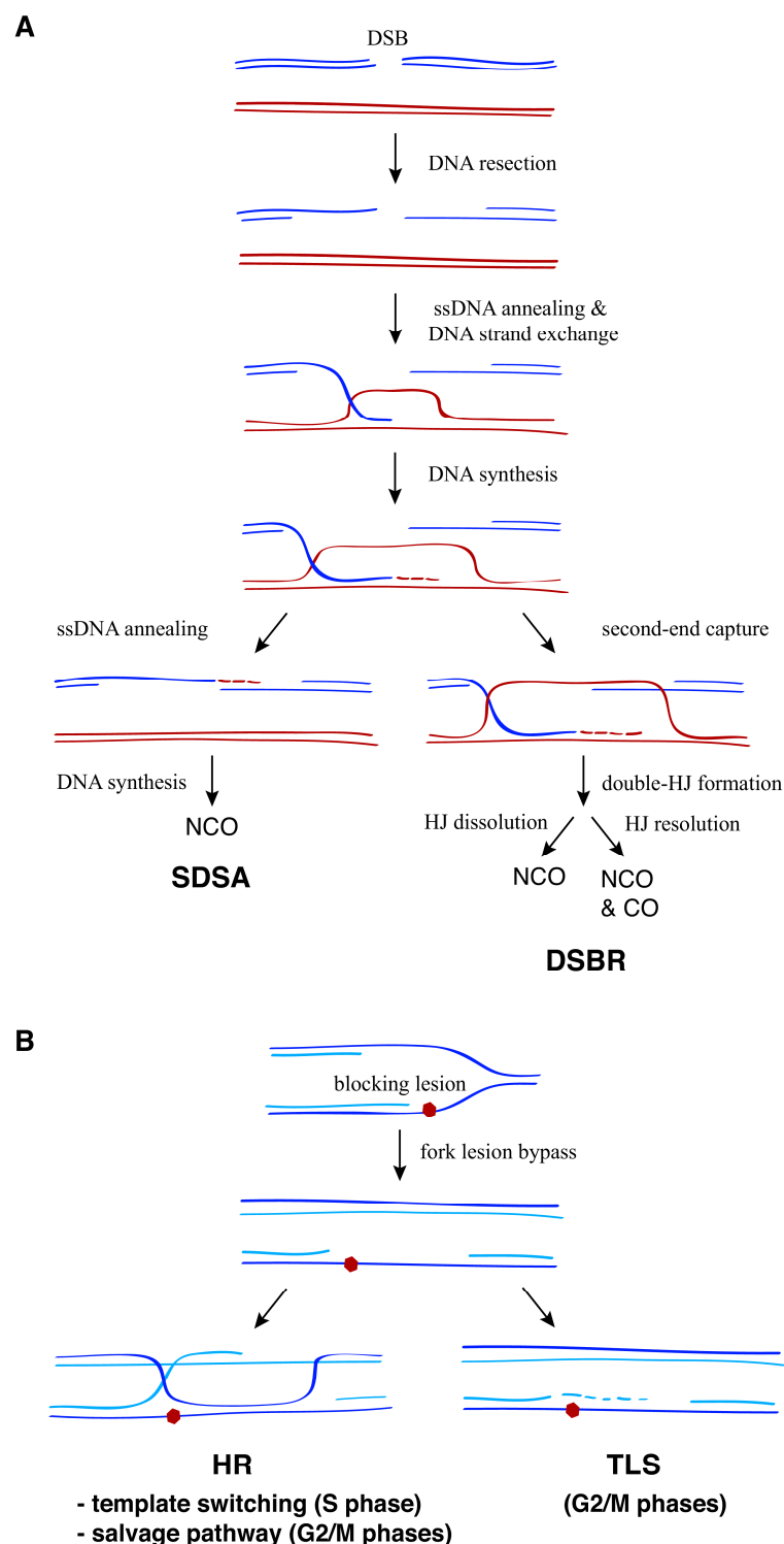
Figure 1. General strategies for the recombinational repair of double-strand breaks (DSBs) and replication associated single-stranded DNA (ssDNA) gaps. (A) In response to DSBs, the 5'-ends of the break are resected, leading to 3'-ended ssDNA molecules that search for and then invade a homologous DNA sequence through Rad51-dependent ssDNA annealing and DNA strand exchange reactions. This generates a D-loop intermediate that can be processed by two major pathways: synthesis-dependent strand annealing (SDSA) or double-strand break repair (DSBR). Whereas SDSA leads to non-crossovers (NCO), the output of DSBR (non-crossover versus crossover) depends on whether the double-Holliday junction (HJ) is dissolved by the STR complex or resolved by DNA structure-specific nucleases. (B) DNA damage tolerance (DDT) mechanisms promote replication fork
