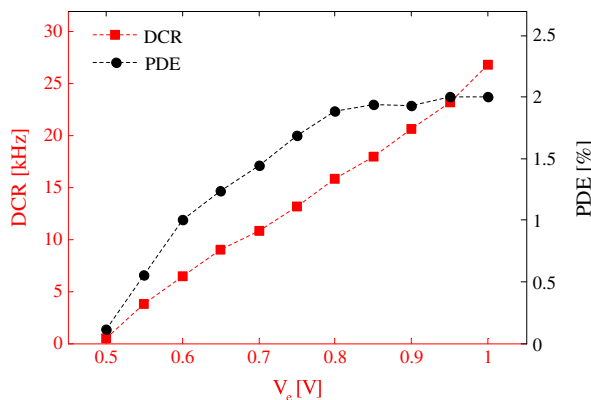
Figure 8. PDE and dark-count rate (DCR) versus V_e at 447 nm wavelength.
