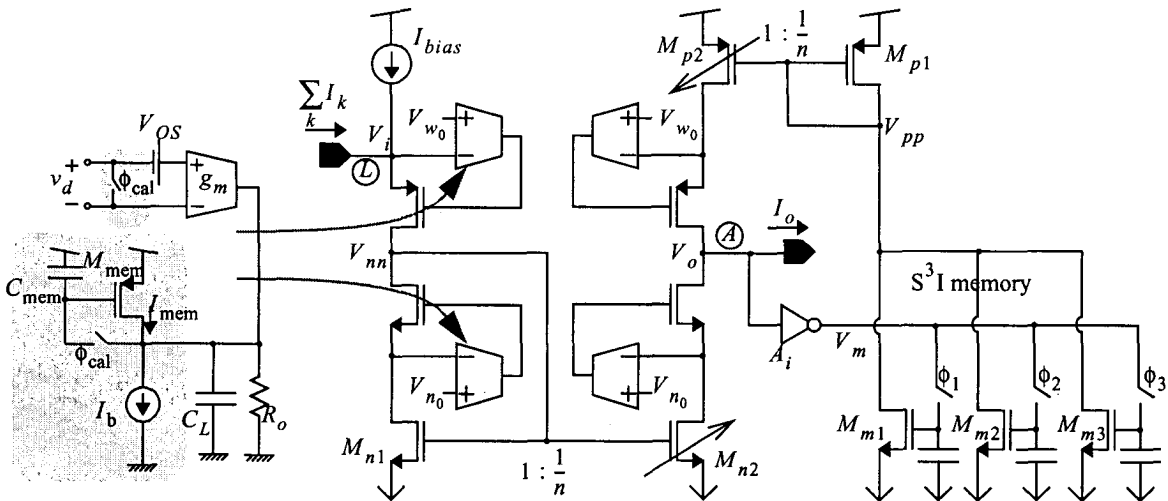
Fig. 5. Input block with current scaling, S 3 I memory and offset-corrected OTA schematic.
