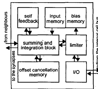
Fig. 4. Internal structure of each CNN layer node.
