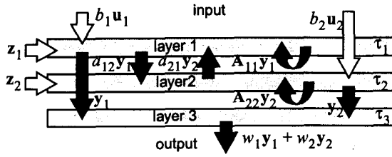
Fig. 2. Diagram of the 2nd-order CNN.
