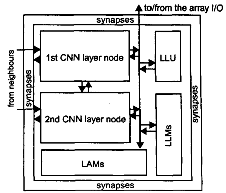
Fig. 3. Conceptual diagram of the basic cell
