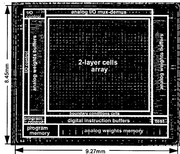
Fig. 6. Microphotograph of the prototype chip.
