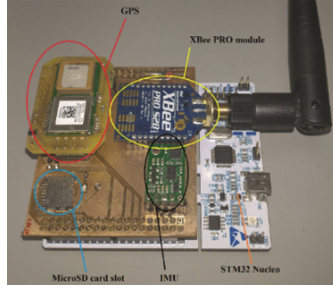
Fig. 2. Collar device prototype
