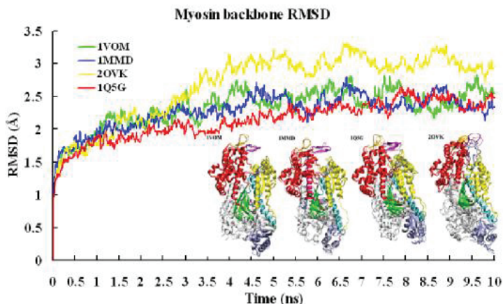
Figure 25: Four myosin structures before and after MD simulations. Different regions of myosin structures are color-coded (Red: upper 50 kDa domain; Yellow: lower 50 kDa domain; Green: \beta -sheet; Orange: loop 4; Purple: CM-loop; Ice blue: converter domain; Cyan: relay-helix; White: others). RMS deviations were drawn as a function to the first 10 ns MD simulations.
