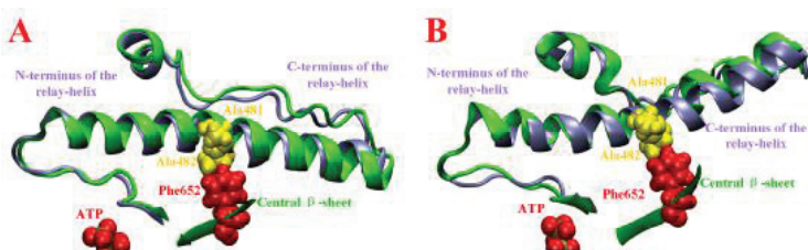
Figure 19: The conformation of myosin relay-helix in the pre-recovery and post-recovery states. A: Pre-recovery conformations of the wild type (Ice blue) and mutant (green) (F481A/F482A). B: Post-recovery conformations of the wild type (Ice blue) and mutant (green) (F481A/F482A).
