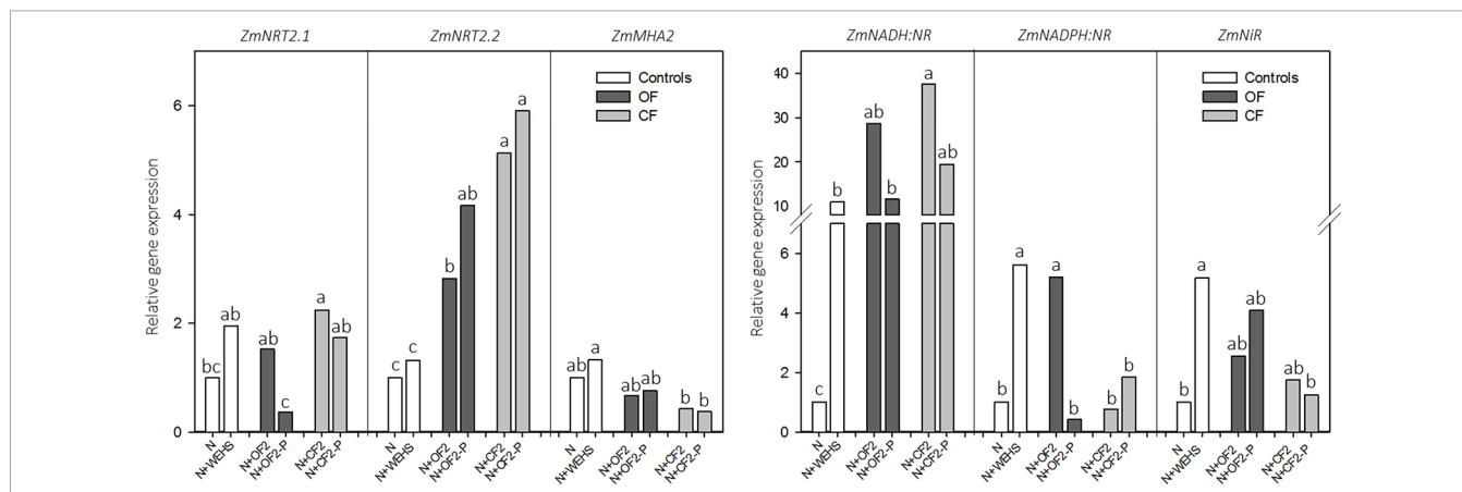
FIGURE 4 | Real-time RT-PCR analyses of the main genes involved in the nitrate acquisition— ZmNRT2.1 and ZmNRT2.2 (coding for two high-affinity nitrate transporters), ZmMHA2 (coding for a PM H + -proton pump), ZmNADPH:NR and ZmNADH:NR (coding for two isoforms of nitrate reductase), and ZmNIR (coding for nitrite reductase)—and performed on roots of maize plants exposed for 2 h to humic substances of different origin isolated in April. White bars , As controls, plants exposed to nutrient solution containing nitrate (0.5 mM Ca(NO 3 ) 2 ) with or without water-extractable humic substances (WEHS) (5 mg C org L -1 ) (N+WEHS or N, respectively). Dark gray bars , Plants exposed to nutrient solution with nitrate and dissolved humic substances (DHS) (5 mg C org L -1 ) isolated from organic farming (OF) soils. Light gray bars , Plants exposed to nutrient solution with nitrate and DHS (5 mg C org L -1 ) isolated from conventional farming (CF) soils. The code name of samples is reported in Figure 1 . Bars with the same letters are not significantly different at p \leq 0.05 .
