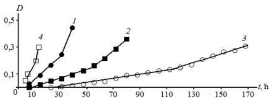
Figure 1. The dependence of optical density on the time and temperature of the test partially synthetic engine oil Mazda Original 10W - 40 SL/CF: 1 - 180 °C; 2 - 170 °C; 3 - 160 °C; 4 - 190 °C.
