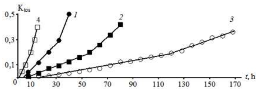
Figure 7. Dependences of the coefficient of thermo-oxidative stability on the time and temperature of testing partially Mazda Original synthetic engine oil: 1 - 180 °C; 2 - 170 °C; 3 - 160 °C; 4 - 190 °C.
