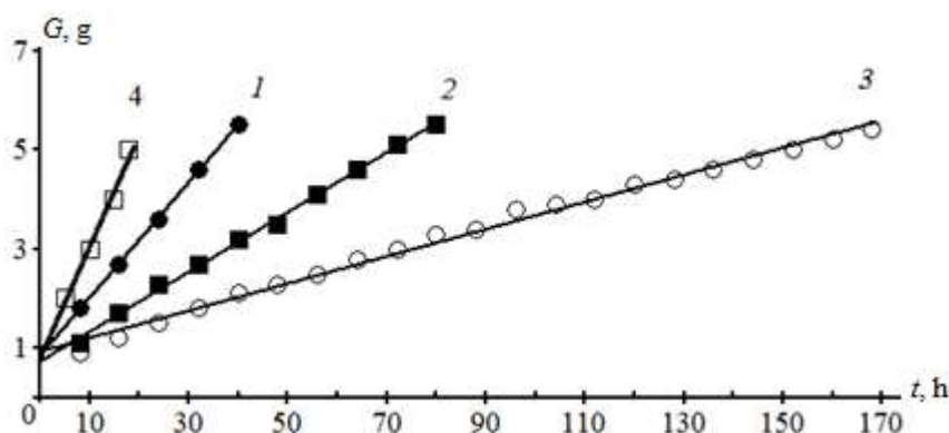
Figure 4. Dependencies of evaporation on the time and temperature of the test of a partially synthetic Mazda Original 10W-40 SL/CF engine oil: 1 - 180 °C; 2 - 170 °C; 3 - 160 °C; 4 - 190 °C.
