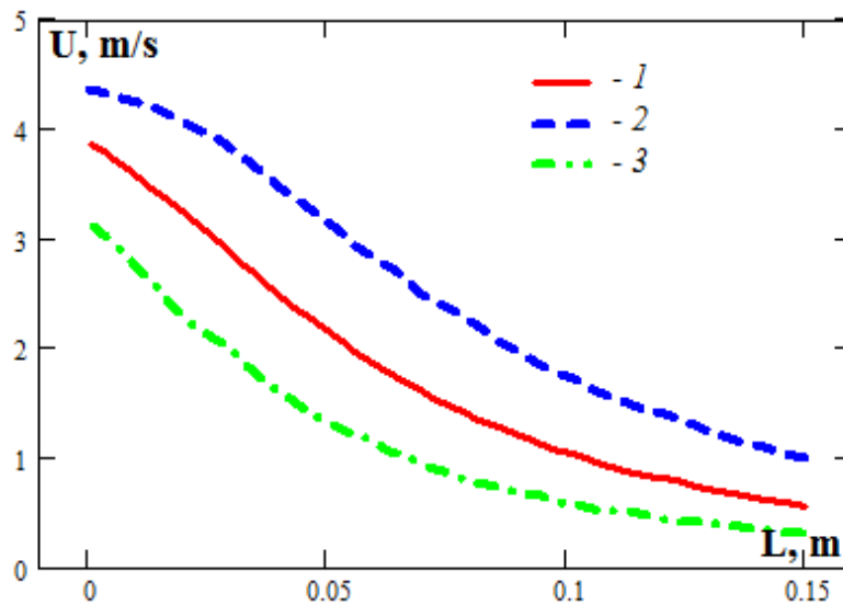
Figure 4. Velocity distribution along the central axis at the different distance from the ventilation channel ( 1 - Q_s/Q_v = 0.5 ; 2 - Q_s/Q_v = 1 ; 3 - Q_s/Q_v = 2 )
