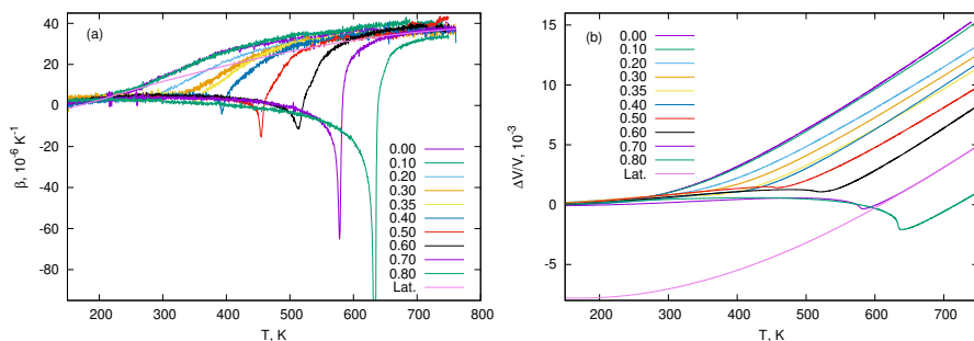
Figure 1. Temperature dependences of the volume thermal expansion coefficient(a) and bulk deformation (b) of solid solutions (1-x)\text{PNN}-x\text{PT} . Lat. — lattice (non-anomalous) component of deformation for the composition with x=0.70 .
