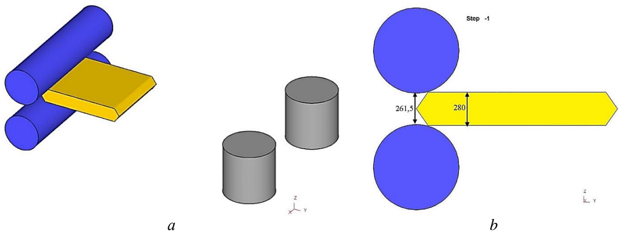
Fig. 1. Three-dimensional model of the ingot and work rolls of the mill (a) and hot rolling scheme (b) slab on an industrial rolling mill QUARTO 2800 with edger rolls
