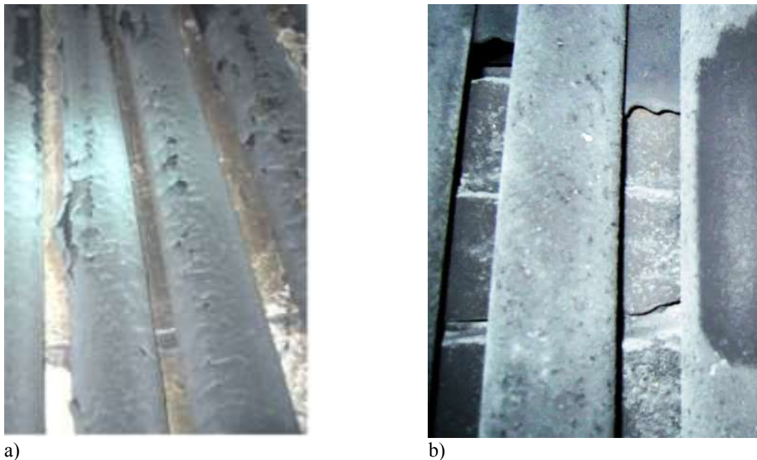
Figure 1. The view of surface of screen tubes: a) before the application of additive; b) after the application of the additive
