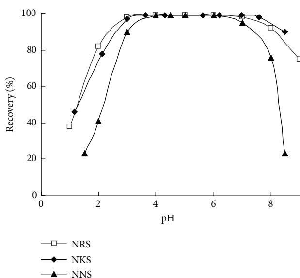
FIGURE 1: Effect of pH on NRS, NKS, and NNS adsorption on \text{SiO}_2 -PHMG as a function of pH. m_{ads} = 0.1 g, C_{OR} = 2.65 \cdot 10^{-5} M, sample volume 10 mL, and shaking time 5 min.
