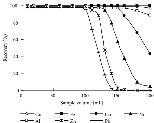
FIGURE 8: The effect of sample volume on metal recoveries for SiO 2 -PHMG-NRS. Mass of adsorbent in the column 0.1 g, pH 6.5, and flow rate 1.5 mL min -1 . Concentration of metals: 200 ng mL -1 of Fe(III), 50 ng mL -1 of Cu(II), Al(III), Zn(II), and 20 ng mL -1 of Co(II), Ni(II), Pb(II).
