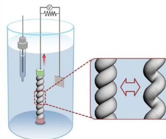
Mechanoelectric conversion
