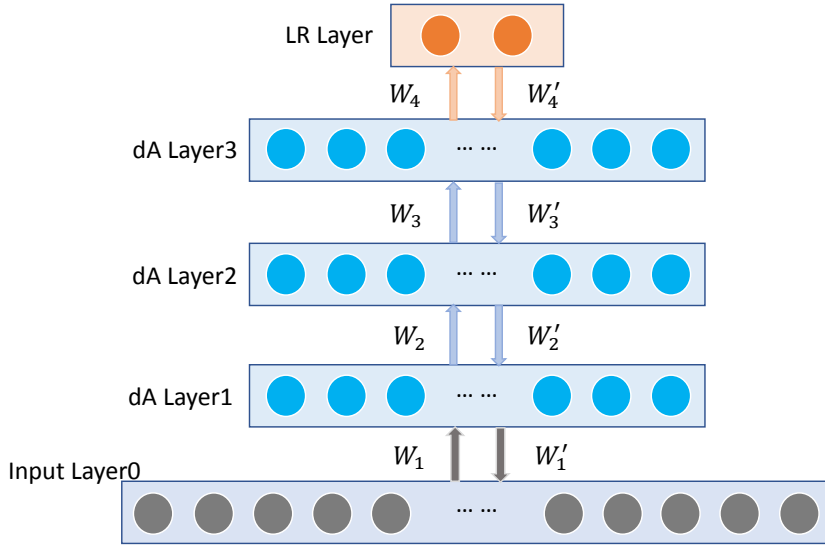
Fig. 3: The Whole Model based on SdA
