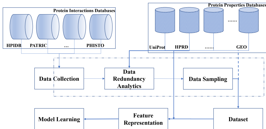
Fig. 1: A Brief Illustration of HP-PPI Framework
