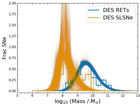
Figure C11: DES RETs compared to DES SLSNe.
