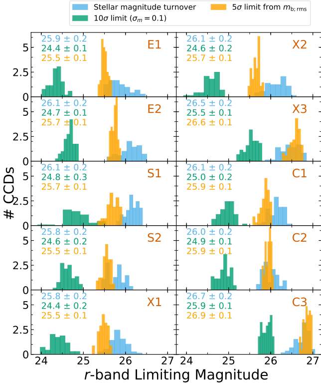
Figure 5. Histograms of the limiting r -band magnitudes for all CCDs in each of the ten SN fields for the MY1 coadd. The extra magnitude of depth in the deeper fields, X3 and C3, is clearly evident. The means and standard deviations of the limiting magnitude distributions are displayed in the upper left corner for each field. While we report 5\sigma limits in this catalogue, we also show 10\sigma limits from magnitude uncertainties (green) for consistency with previous catalogues. Summaries of the coadd properties are given in Table A1.
