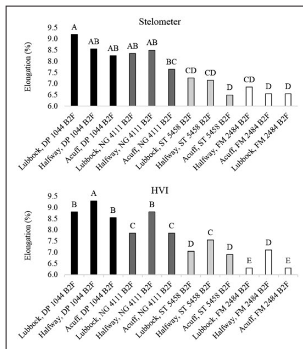
Figure 7. Elongation means for different cultivars and locations measured by the Stelometer and the High Volume Instrument (HVI). Means not sharing any letter are significantly different by Tukey's test at the 5% level of significance.
