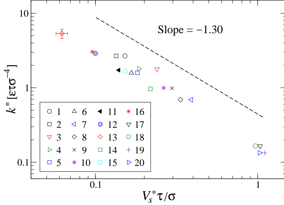
FIG. 7: (Color online) The normalization parameters V_s^* (in units of \sigma/\tau ) and k^* (in units of \varepsilon\tau\sigma^{-4} ) used to fit the data in Fig. 6 to Eq. (7). The indices in the inset denote systems listed in Table I. The dashed line with a slope -1.30 is shown for reference.
