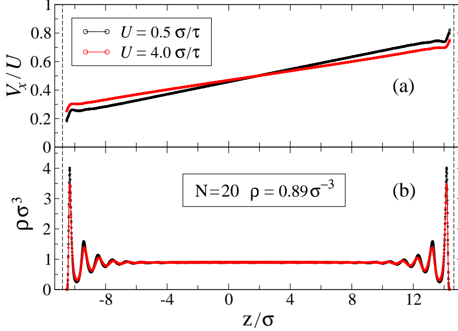
FIG. 3: (Color online) Averaged normalized velocity (a) and density (b) profiles across the channel for the upper wall speeds U = 0.5 \sigma/\tau and U = 4.0 \sigma/\tau . The uniform monomer density of the polymer melt N = 20 away from the walls is \rho = 0.89 \sigma^{-3} (system 5 in Table I). The vertical axes indicate the location of the fcc lattice planes (at z/\sigma = -11.30 and 15.14 ) in contact with the fluid. The dashed lines at z/\sigma = -10.80 and 14.64 denote reference planes for computing the slip length.
