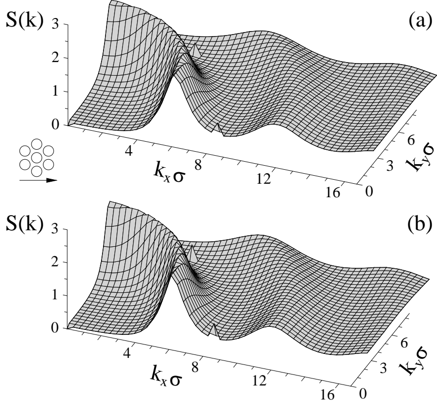
FIG. 10: Two-dimensional structure factor S(k_x, k_y) computed in the first fluid layer for N = 1 and U = 0.05 \sigma/\tau [systems (a) 19 and (b) 17 in Table I]. The wall-fluid interaction energy is (a) \varepsilon_{\text{wf}} = 0.3 \varepsilon and (b) \varepsilon_{\text{wf}} = 0.4 \varepsilon . The shear flow direction (denoted by the horizontal arrow) is parallel to the [11\bar{2}] orientation of the (111) face of the fcc wall lattice (open circles).
