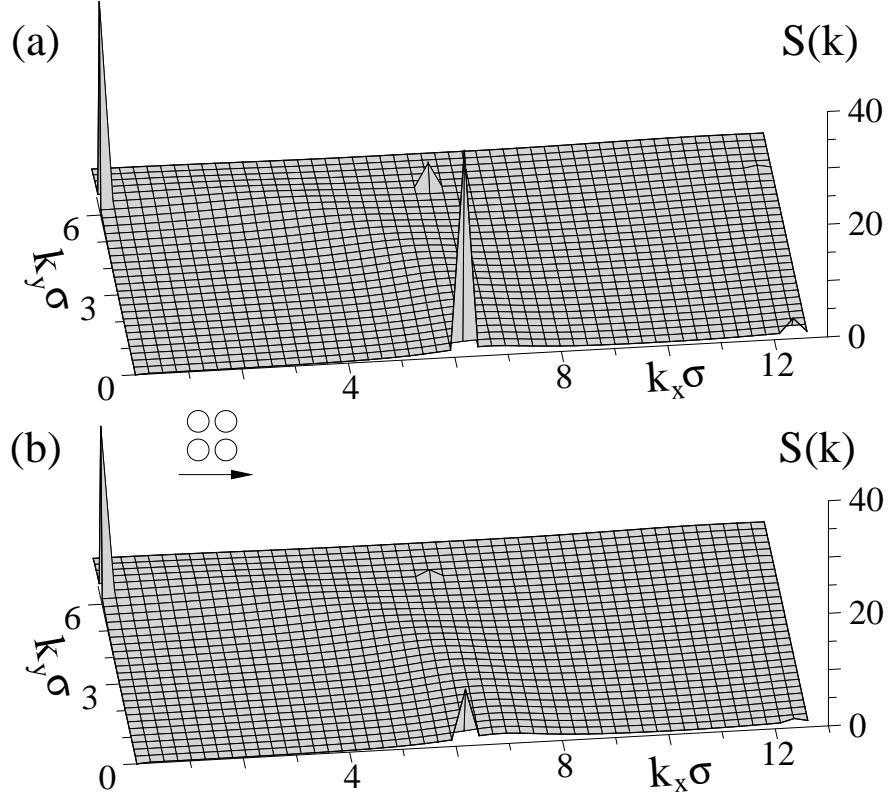
FIG. 12: Structure factor S(k_x, k_y) computed in the first fluid layer for N = 20 polymer system 12 (see Table I). The upper wall speed and slip velocity are (a) U = 0.05 \sigma/\tau and V_s = 0.012 \sigma/\tau and (b) U = 2.0 \sigma/\tau and V_s = 0.51 \sigma/\tau , respectively. The horizontal arrows denote the shear flow direction with respect to the orientation of the (001) face of the bcc wall lattice (open circles).
