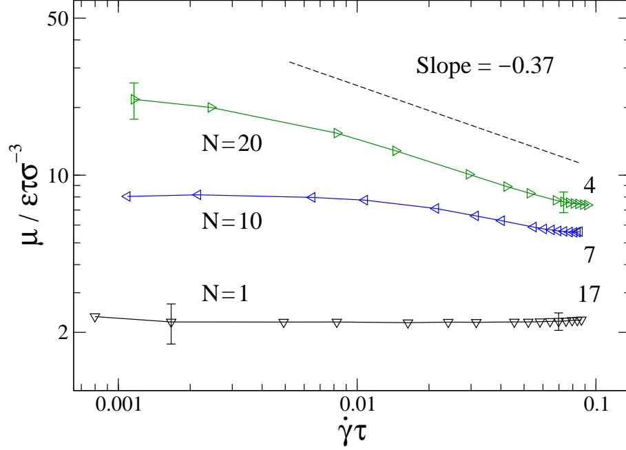
FIG. 4: (Color online) Shear rate dependence of the fluid viscosity \mu (in units of \varepsilon\tau\sigma^{-3} ) for the indicated systems (listed in Table I). The dashed line with a slope -0.37 is shown for reference.
