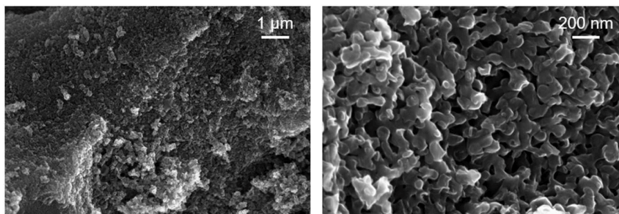
FIGURE 2 | SEM images of the heat-treated carbon replica at two different magnifications.
