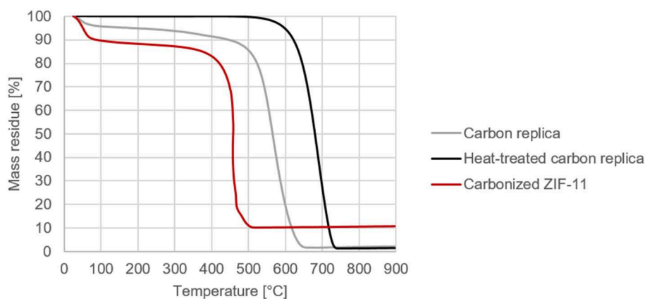
FIGURE 6 | Comparative decomposition curves of carbon replicas in air (programmed temperature ramp from ambient conditions to 900^\circ\text{C} at 10^\circ\text{C} per min in a TG setup).
