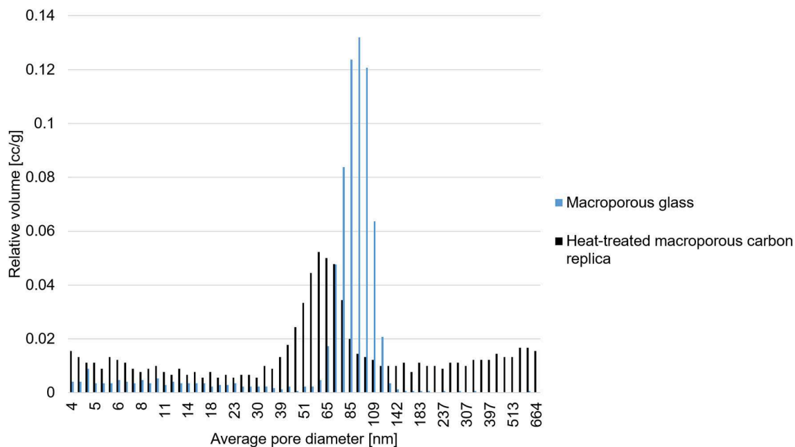
FIGURE 3 | Estimated pore size distribution in the mesoporous and macroporous size range.
