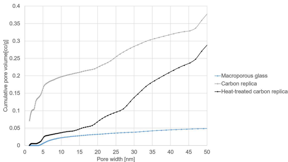
FIGURE 5 | Pore size distributions in the micro- and mesoporous range from DFT modeling of N_2 sorption isotherms at -195.8^\circ\text{C} .
