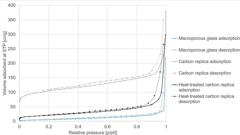
FIGURE 4 | N_2 sorption isotherms at -195.8^\circ\text{C} of macroporous glass, its carbon replica, and the heat-treated carbon replica.
