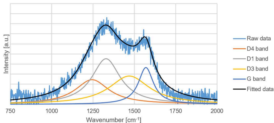
FIGURE 7 | Raw and fitted Raman spectral data of the carbon replica.
