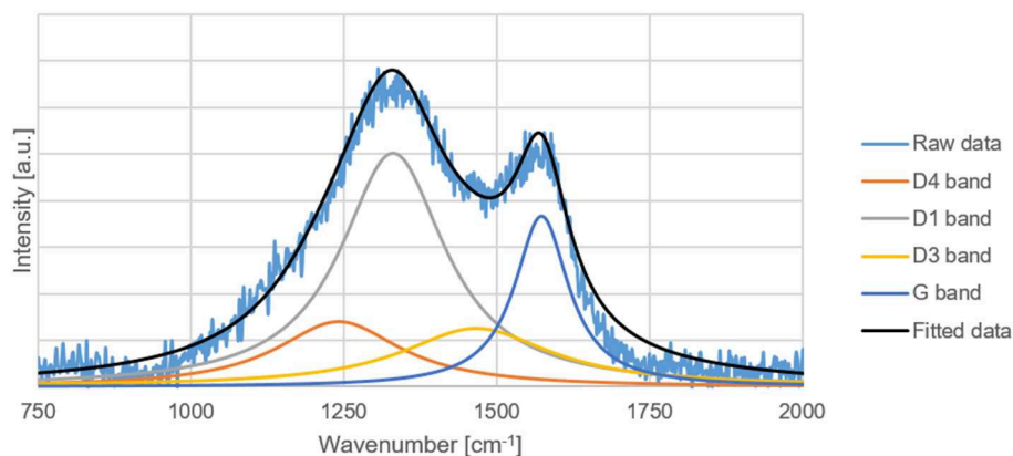
FIGURE 8 | Raw and fitted Raman spectral data of the heat-treated carbon replica.
