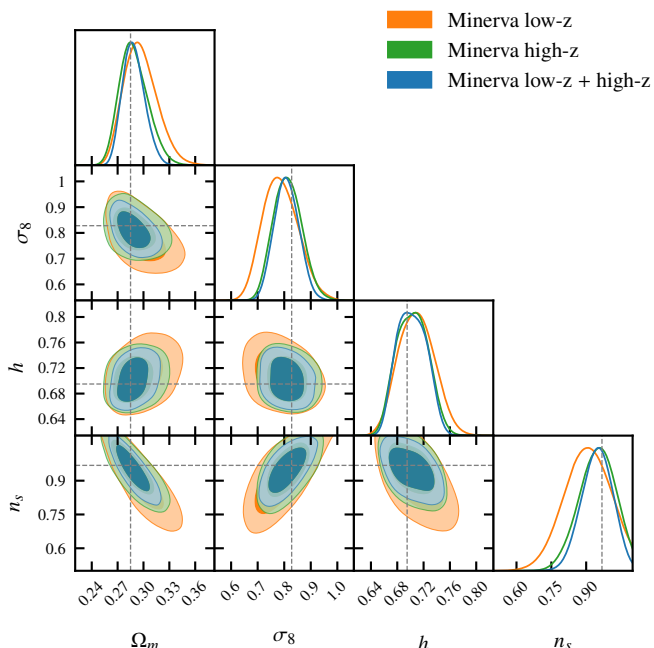
Fig. A.1. Cosmological parameters inferred from the Minerva mocks for low-redshift sample (orange), high-redshift sample (green), and joint analysis of both samples (blue). The true cosmology is indicated with dashed lines.
