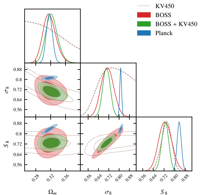
Fig. 4. Constraints on flat \Lambda CDM when combining BOSS DR12 with KV450 (green). The red and blue contours are the same as Fig. 3 and denote the constraints from BOSS and Planck alone. The constraints from KV450 are shown with dashed lines.
