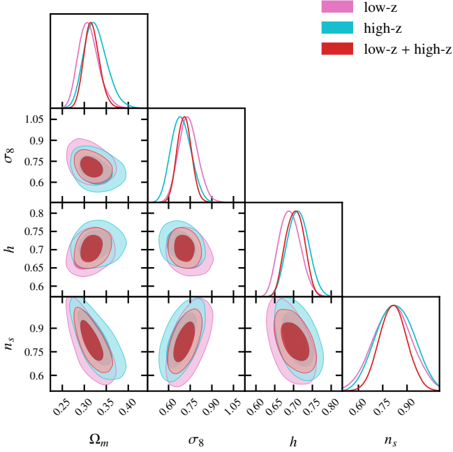
Fig. C.1. Constraints on flat \Lambda CDM derived from BOSS DR12 correlation function wedges using only the low-redshift bin (pink), only the high-redshift bin (cyan), and the joint constraints used in the main analysis (red).
