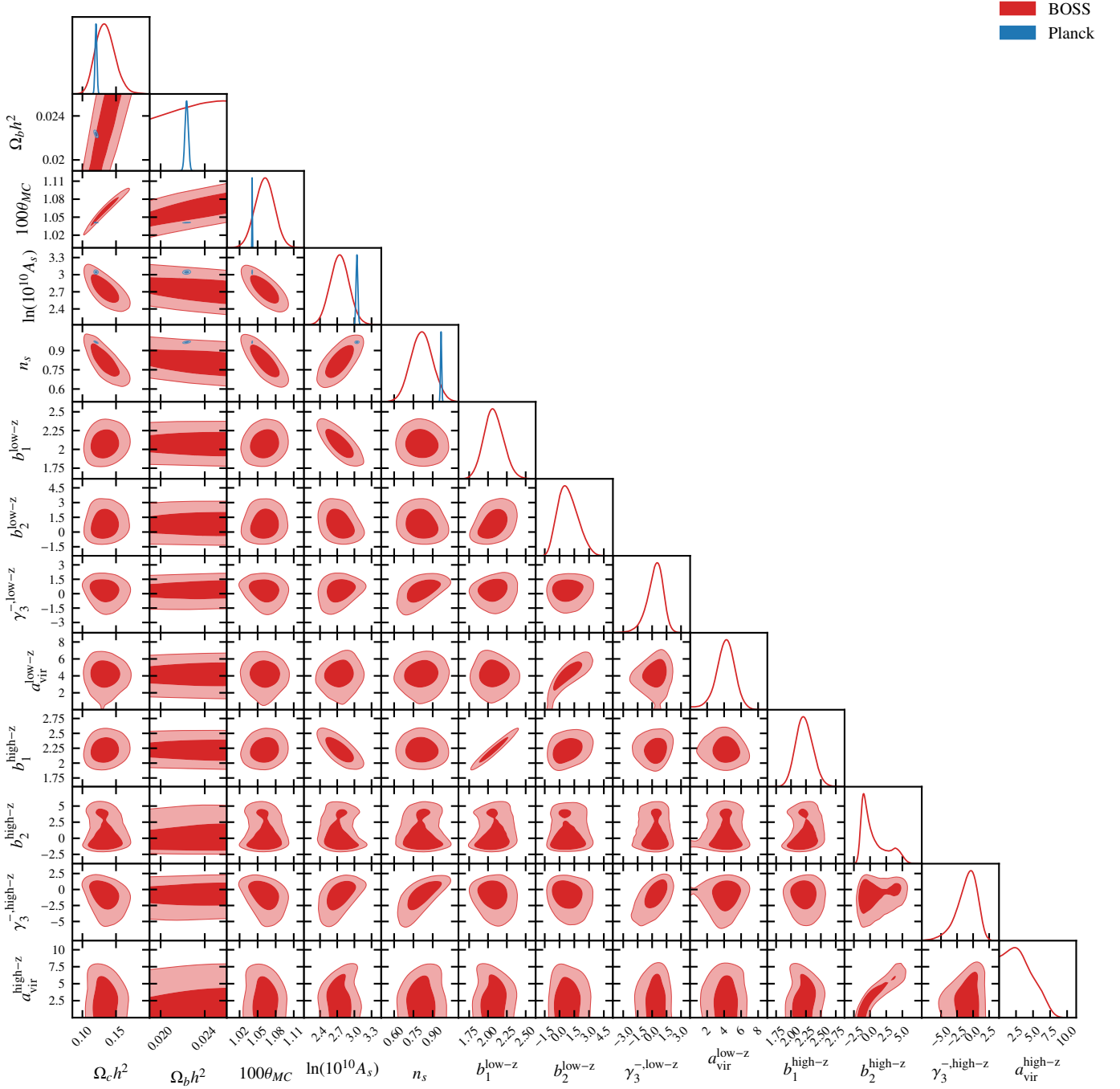
Fig. B.1. Posterior distributions for all sampled parameters in our main analysis. The posteriors derived from the BOSS clustering wedges are shown in red, while those from Planck 2018 are shown in blue.
