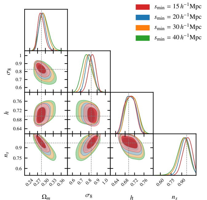
Fig. 1. Cosmological parameters inferred from the Minerva mocks for different choices of the minimum separation scale used in the measurement. The true cosmology is indicated with dashed lines, while the cosmological constraints are shown in red ( s_{\min} = 15 h^{-1} Mpc), blue ( s_{\min} = 20 h^{-1} Mpc), orange ( s_{\min} = 30 h^{-1} Mpc), and green ( s_{\min} = 40 h^{-1} Mpc).
