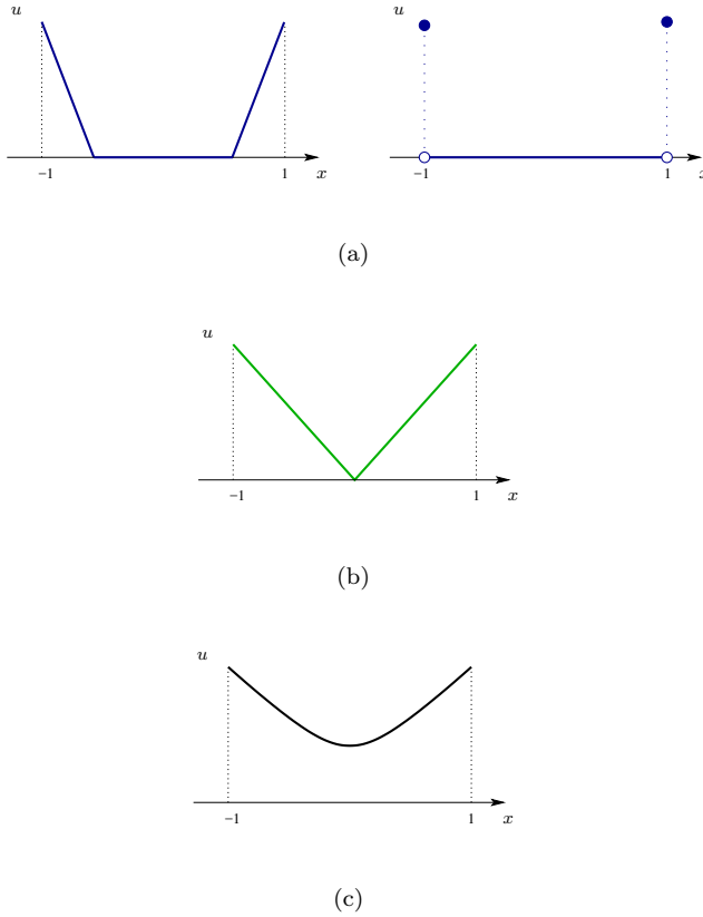
FIGURE 8. Singular solutions to Equation (2.9), as specified in Definition 4.1: (a) type I-solutions for \lambda = \mathcal{O}(\varepsilon) (left panel) and \lambda = \mathcal{O}(1) (right panel), (b) type II-solutions, and (c) type III-solutions.
