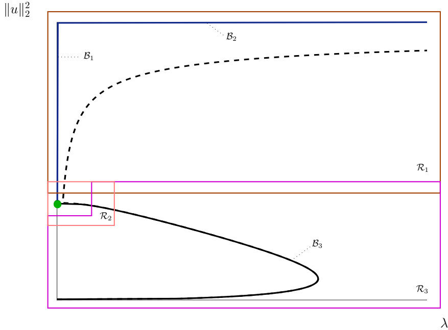
FIGURE 9. Covering of the bifurcation diagram for the boundary value problem \{(2.9),(2.10)\} by three overlapping regions \mathcal{R}_1 (brown), \mathcal{R}_2 (pink), and \mathcal{R}_3 (magenta), for \varepsilon positive and small. (For improved visibility, the regions have been extended slightly below \|u\|_2^2 = 0 , above \|u\|_2^2 = 2 , and to negative \lambda , respectively; also, we recall Remark 4.3 with regard to the interpretation of \|u\|_2^2 in this context.) The branches of solutions to the boundary value problem \{(2.9),(2.10)\} for \varepsilon = 0.01 (dotted curve) and \varepsilon = 0 (solid curve) are also displayed. In \mathcal{R}_3 , these branches overlap almost entirely. For \varepsilon = 0 , the blue branch reduces to the union of a vertical part \mathcal{B}_1 , corresponding to \lambda = \mathcal{O}(\varepsilon) , and a horizontal part \mathcal{B}_2 which corresponds to \lambda = \mathcal{O}(1) . The green dot at B represents the singular solution of type II for \lambda = 0 that is labeled d in Figure 2(a). The black curve, corresponding to the branch of solutions to the non-regularized model, is labeled \mathcal{B}_3 . In the limit as \varepsilon \rightarrow 0 , \mathcal{R}_2 shrinks to a segment on the \|u\|_2^2 -axis that contains the point B , cf. (4.2), while region \mathcal{R}_3 grows to a rectangle minus a smaller segment on the \|u\|_2^2 -axis containing the point B ; recall (4.3).
