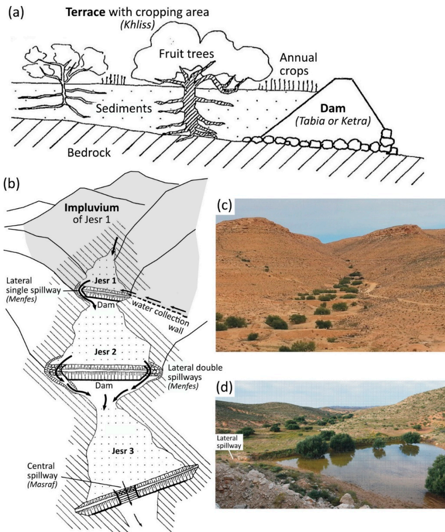
Figure 2. (a) View of a Jessour, adapted from Bonvallot [5]; (b) general view of Jessour with lateral single spillway (Jesr 1), double spillway (Jesr 2) and central spillway (Jesr 3), adapted from Bonvallot [5]; (c) Jessour alignment, note the contrast between arid barren slopes and the bottom of the thalweg in the Jessour (photo: T. Ben Fraj) and (d) Jessour retaining part of the rainwater (photo: Tarek Ben Fraj, taken on 22 November 2017 in the Matmata region).
