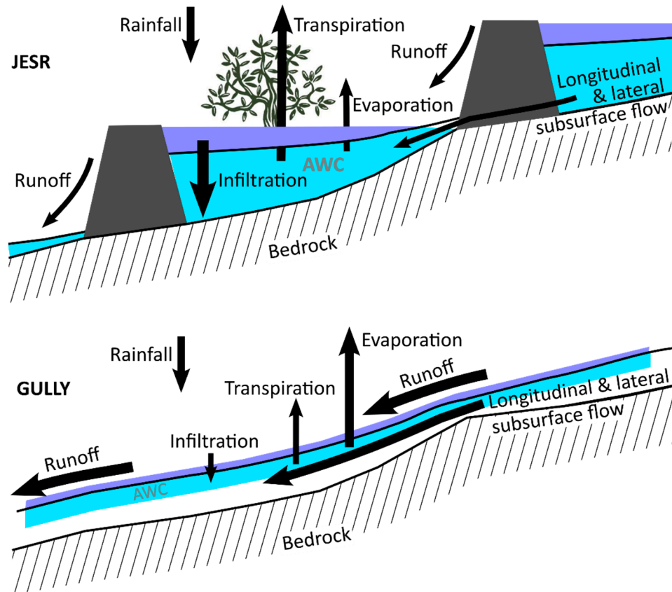
Figure 11. Schematic water balance for the Jesr and the gully. Turquoise: infiltrated water and subsurface flow and blue: surface runoff.
