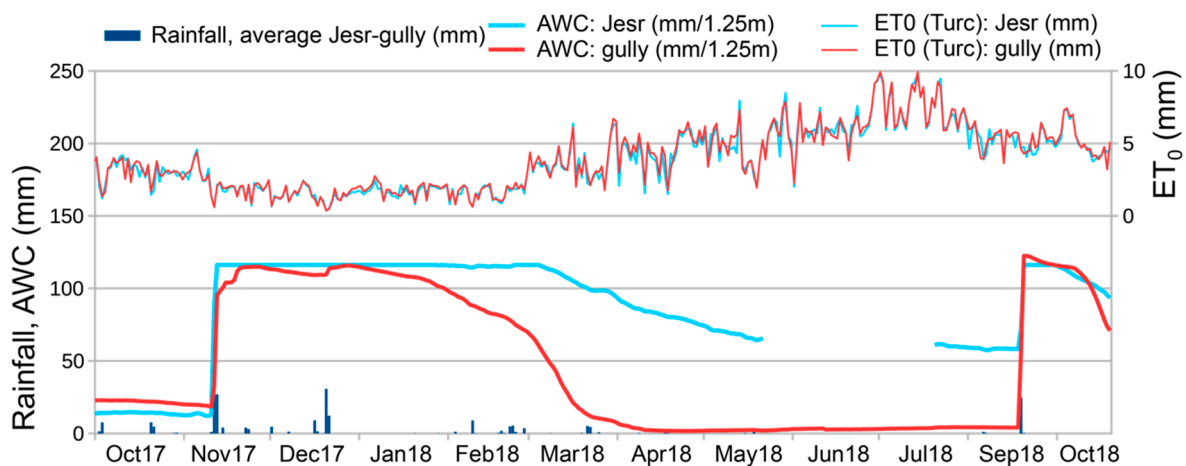
Figure 9. Evolution of available water capacity (AWC) and potential evapotranspiration ( \text{ET}_0 ) in the Jesr and the gully.
