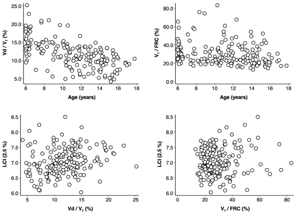
Supplemental Figure 2: Association of V_d/V_T (%) and V_T/FRC (%) with age, and association of LCI 2.5% with V_d/V_T (%) and V_T/FRC (%) in 180 healthy children.
