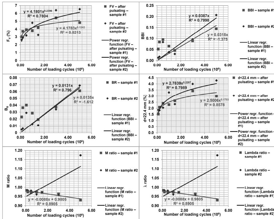
Fig. 3. Results of laboratory dynamic pulsating test ( F_v , BBI, B_R , d < 22.4 mm, M ratio, \lambda ratio parameters as a function of number of loading cycles)
