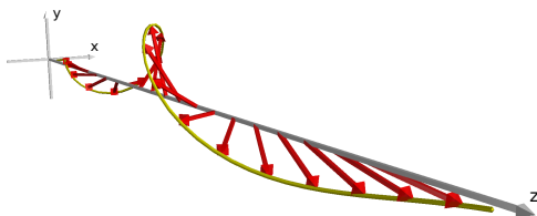
FIG. 1. High-field domain wall with tail-to-tail boundary conditions. The envelope (yellow curve) of the magnetisation (red arrows) indicates a helical as opposed to planar profile. The asymptotic sense and pitch of the helix may be interpreted in terms of the chirality and wavelength of entrained spin waves.
