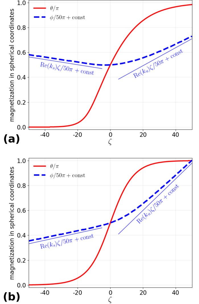
Supplementary Figure 1. Polar coordinates \theta and \phi of the emergent high-field profile along with asymptotic wave numbers (the real parts of k_{s,u} in Eq. (S1)), which determine the rate of twisting in \phi in the tails. In (a) (cf Fig. 2a), the tails have opposite chirality, while in (b) (cf Fig. 2b), the tails have the same chirality. The asymptotic approach is slower in the unstable tail, due to the asymptotic behaviour \eta \sim (c_1 + c_2\zeta)e^{ik_u\zeta} as \zeta \rightarrow +\infty . The parameters in (a) and (b) are the same as in Fig. 2a and Fig. 2b respectively.
