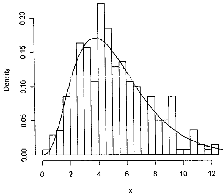
Figure 4: Frequency distribution of sinuosity index of TC tracks; n = 288 .
