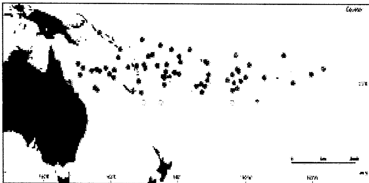
Figure 4(a): Category 1 - tropical cyclone with straight track.
