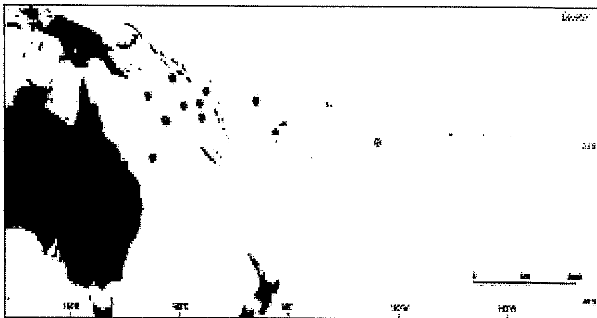
Figure 4(e): Category 5 - tropical cyclone with convoluted track.
