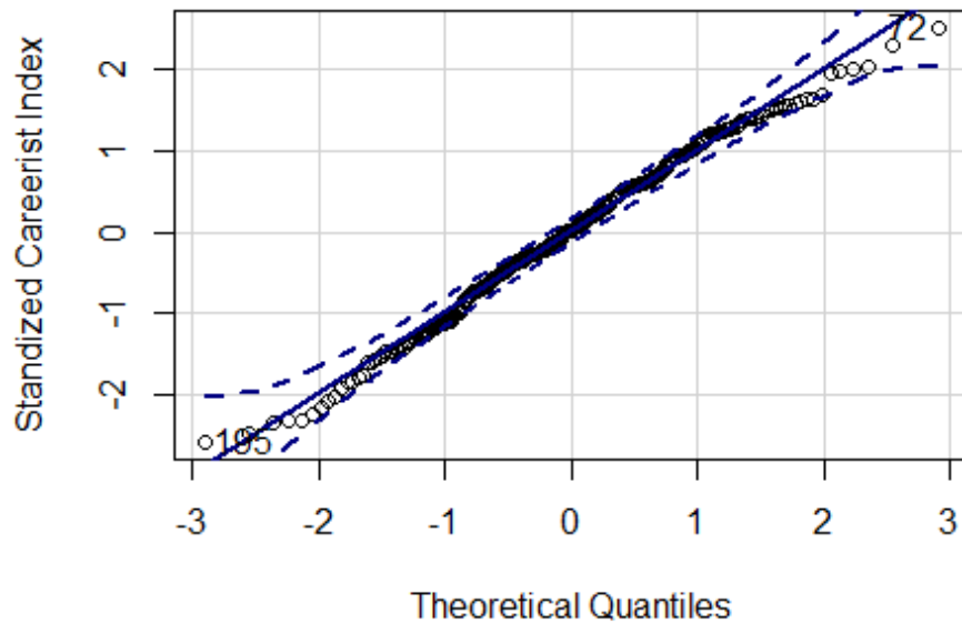
Figure 2: Quantile Comparison Plot for the Standardized Composite Career Politician Index
