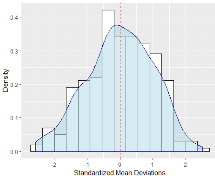
Figure 1: Standardized Composite Career Politician Index Histogram with Superimposed Density Plot
