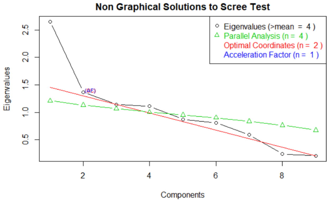
Figure 3: Eigenvalue Plot per Principal Component - Only 1st PC provides meaningful reduction in variance
