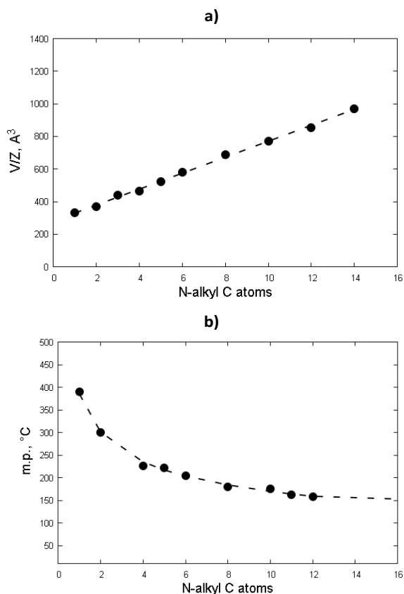
Fig. 2 a) The regular change of the (temperature-corrected) V/Z_{298} values for the entire NDix series (x=1-14). b) melting points of the NDix materials vs n-alkyl C atoms. Data were fit by a phenomenological exponential law:
