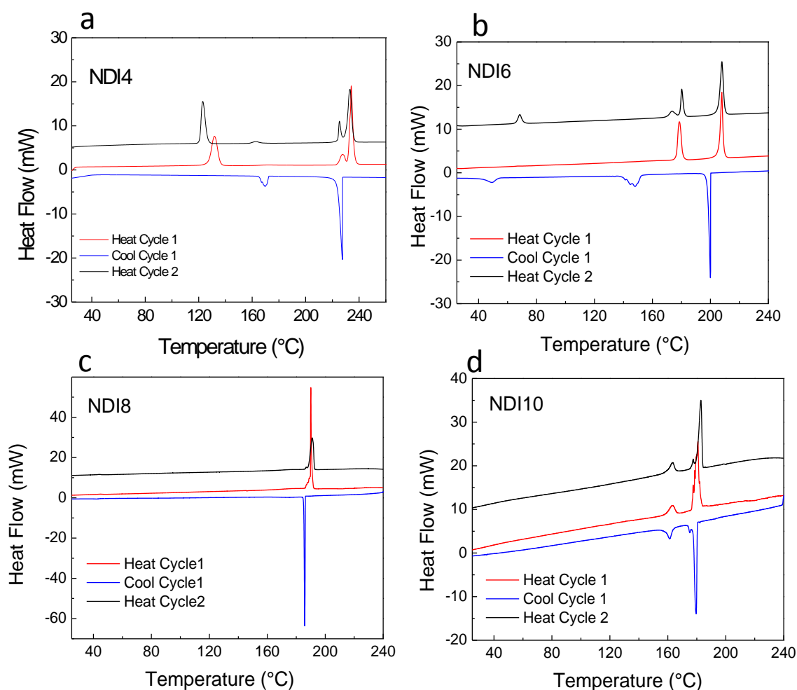
Fig. 6 DSC traces measured on the pristine NDI x (x = 4, 6, 8 and 10) powders, upon heating, subsequent cooling and second heating (red, blue and black traces, respectively).
