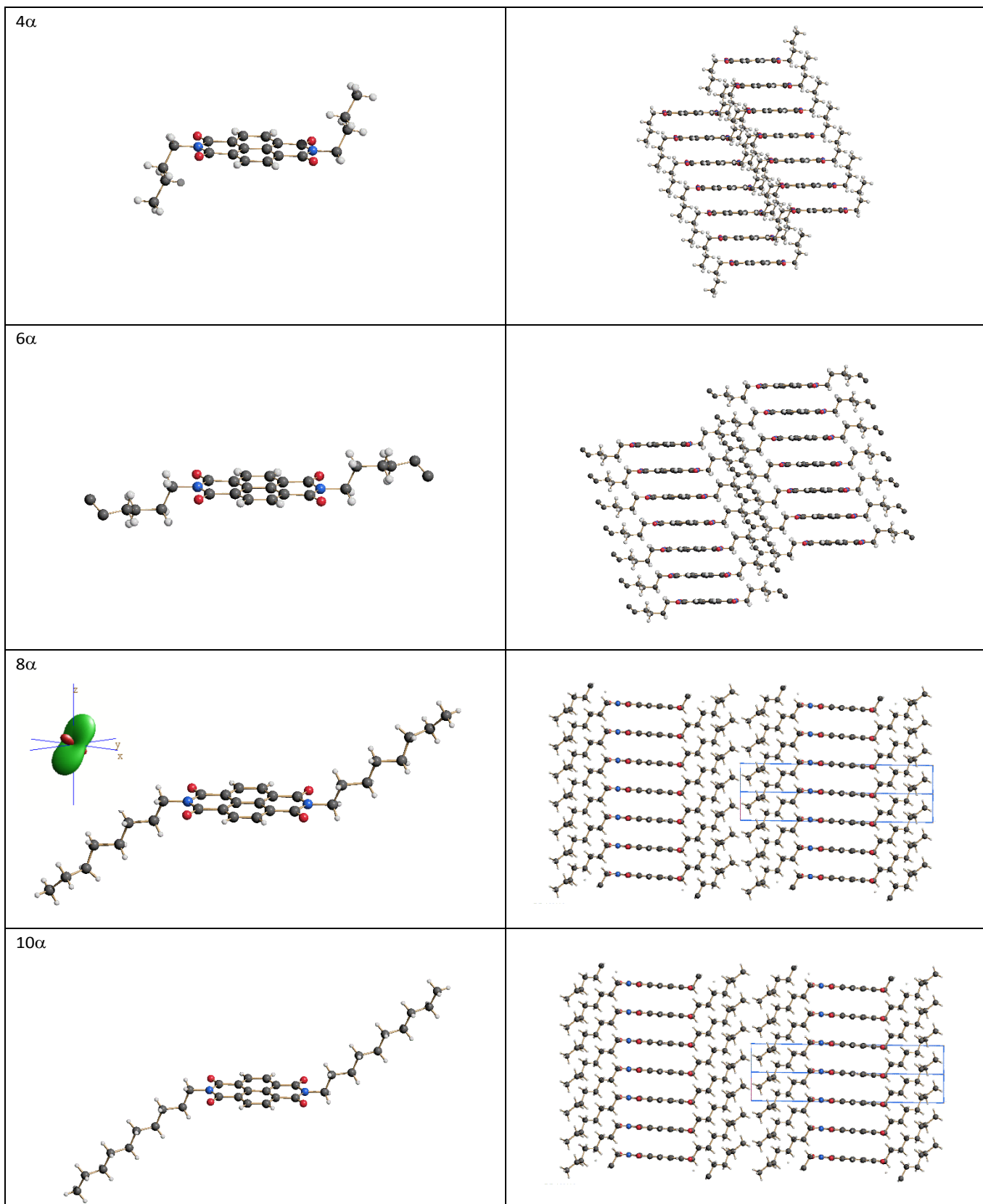
Fig 1 Left: sketches of the molecular geometry of 4 \alpha 13b , 6 \alpha , 31 8 \alpha and 10 \alpha (top to bottom). Color codes: C (grey), N (blue), O (red), H (white). Drawn by SCHAKAL. 32 Due to some alkyl chain disordering in 6 \alpha , some of the alkyl H atoms have not been inserted. The inset in the panel of 8 \alpha shows the highly anisotropic shape drawn from the thermal expansion coefficient for NDI8, heated from RT to 175°C. Right: sketches of the corresponding molecular packing.
