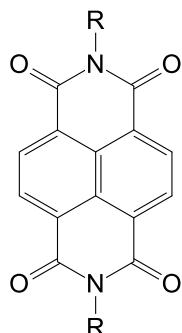
Chart I. Chemical structure of NDI x molecules.
