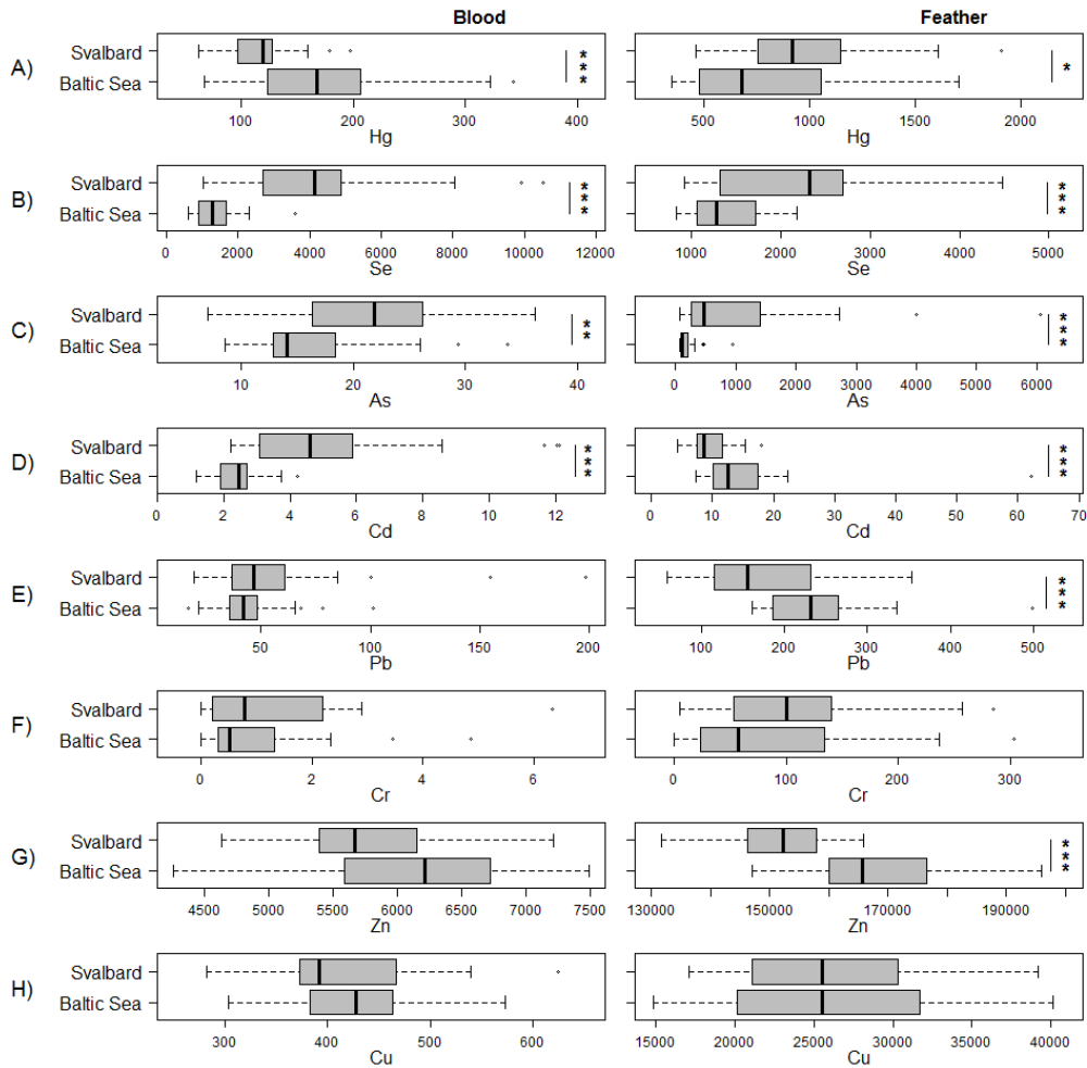
Figure 2: Box plots with blood (left) and feather (right) concentrations ( \mu\text{g}/\text{kg} ww) of A) mercury (Hg), B) selenium (Se), C) arsenic (As), D) cadmium (Cd), E) lead (Pb), F) chromium (Cr), G) zinc (Zn) and H) copper (Cu) in female eiders from Svalbard (upper box) and the Baltic Sea (lower box). The plots show medians (thick vertical lines in boxes) along with the interquartile range (IQR, box), maximum and minimum values within 1.5 IQR (whiskers) and values outside IQR (outliers). P-values from linear models (see text) are indicated by stars (*) to the right of the boxes, where p < 0.001 is indicated by ***, p < 0.01 by ** and p < 0.05 by *.
