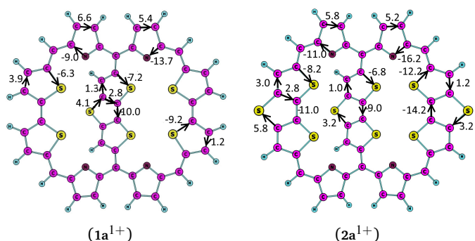
Fig. 8 The strengths (in nA/T) of the current pathways of 1a^{1+} and 2a^{1+} calculated at the B3LYP/def2-TZVP level of theory.
