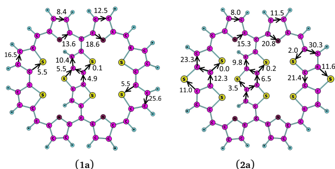
Fig. 3 The strengths (in nA/T) of the current pathways of 1a and 2a calculated at the B3LYP/def2-TZVP level of theory.
