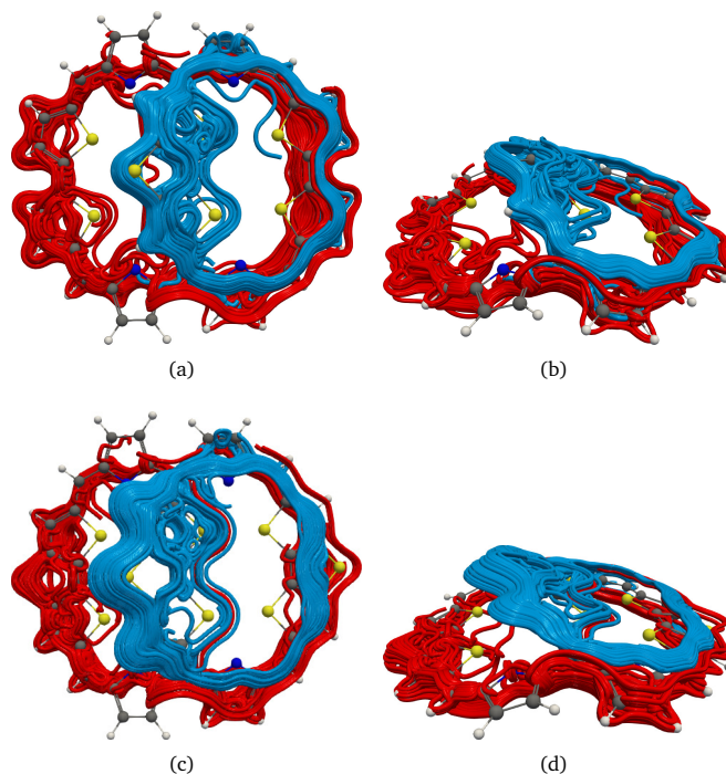
Fig. 2 The magnetically induced ring currents of the two rings of 1a are shown in (a) and (b). Figures (c) and (d) show the corresponding ring currents of 2a . The visualization has been done with the 3D streamline visualization plugin of ParaView using a sphere radius of 0.4 bohr. For streamlines depicted in blue, the inspection sphere was placed 1 bohr above the fusing carbon atom at the DDT bridge, while for the red streamlines the sphere was placed 1 bohr below the neighboring carbon atom to the left of the junction.
