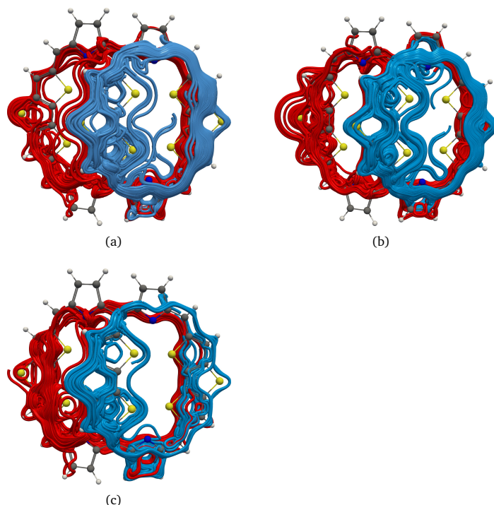
Fig. 5 The 3D streamlines for (a) the total current density, (b) the \alpha contribution and (c) \beta contribution to the total current density of 2a^{2+} . The streamlines depicted in blue was obtained with the inspection sphere 1 bohr above the fusing carbon atom at the DDT bridge, while for the red streamlines the sphere was placed 1 bohr below the neighboring carbon atom to the left of the junction.
