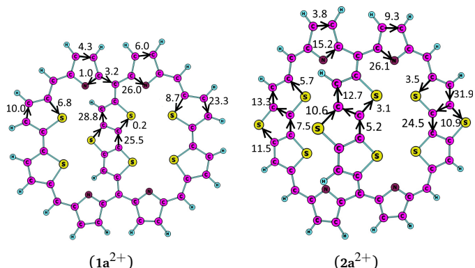
Fig. 6 The strengths (in nA/T) of the current pathways of the triplet state of the 1a^{2+} and 2a^{2+} dications calculated at the B3LYP/def2-TZVP level of theory.
