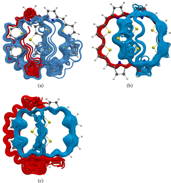
Fig. 7 Calculated current density represented as 3D streamlines for (a) the total current density, (b) the \alpha contribution and (c) the \beta contribution to the current density of 1a^+ . For streamlines depicted in blue the inspection sphere was placed 1 bohr above the fusing carbon atom at the DDT bridge, while for the red streamlines the sphere was placed 1 bohr below the neighboring carbon atom to the left of the junction.
