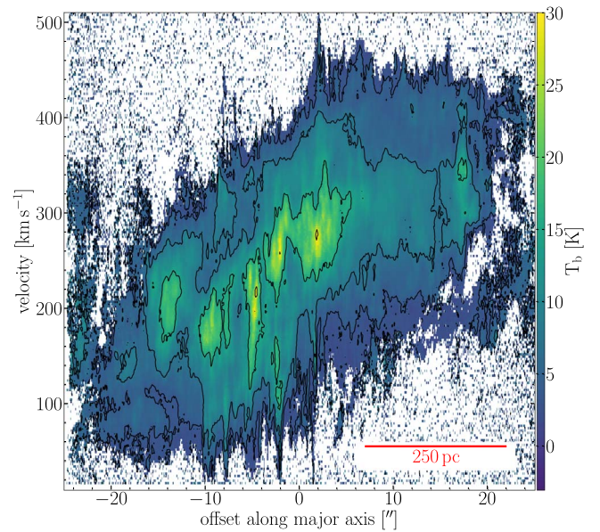
Figure 3. CO(3–2) position–velocity diagram of NGC 253 along the major axis centered on the kinematic center averaged over the full width of the field of view ( \sim 30'' ). Pixels below 3\sigma are masked and contours are drawn at 10\sigma , 20\sigma , 40\sigma , 80\sigma with an rms noise of \sigma = 0.37 K. Note the vertical spikes indicating high-velocity dispersion due to outflowing gas.
