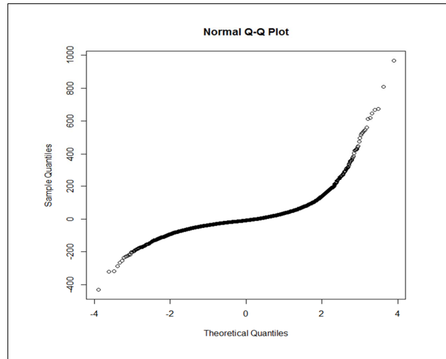
Fig. 3. Quantile-Quantile Plot for Investigating Normality
