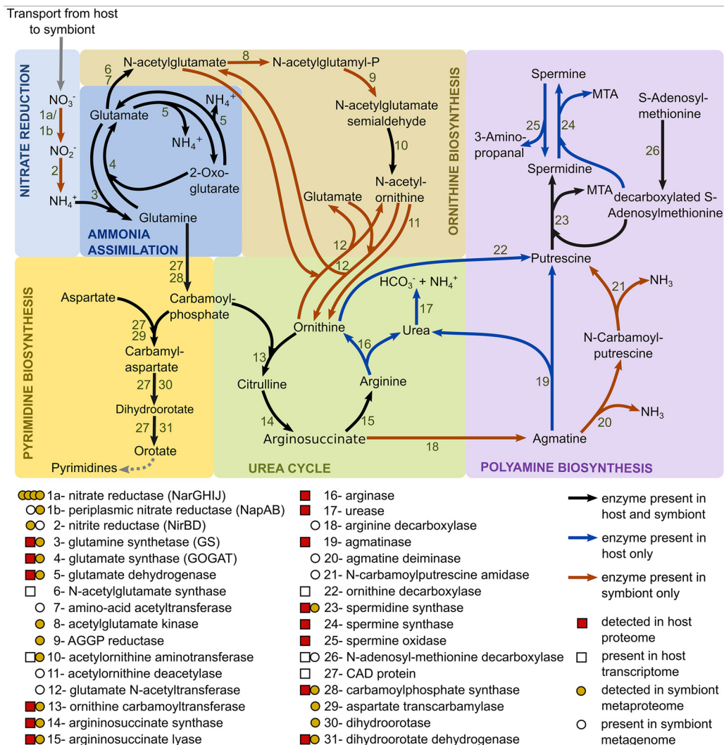
FIG 4 Main nitrogen metabolic pathways in Riftia symbiosis. AGGP reductase, N-acetyl-gamma-glutamyl-phosphate reductase; CAD protein, multifunctional carbamoyl-phosphate synthetase 2, aspartate transcarbamoylase, and dihydroorotase protein; MTA, 5'-methylthioadenosine. Note that the symbiont might also be capable of nitrate respiration (25, 60), which is not depicted here.
